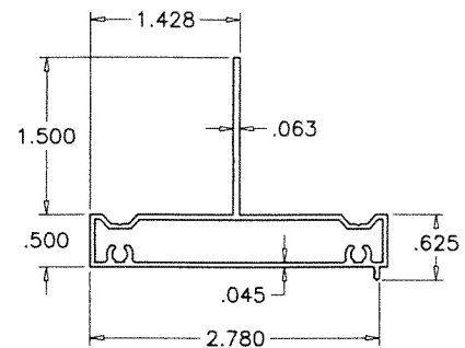
E6 FLUSH FRAME ADAPTER WITH FIN
