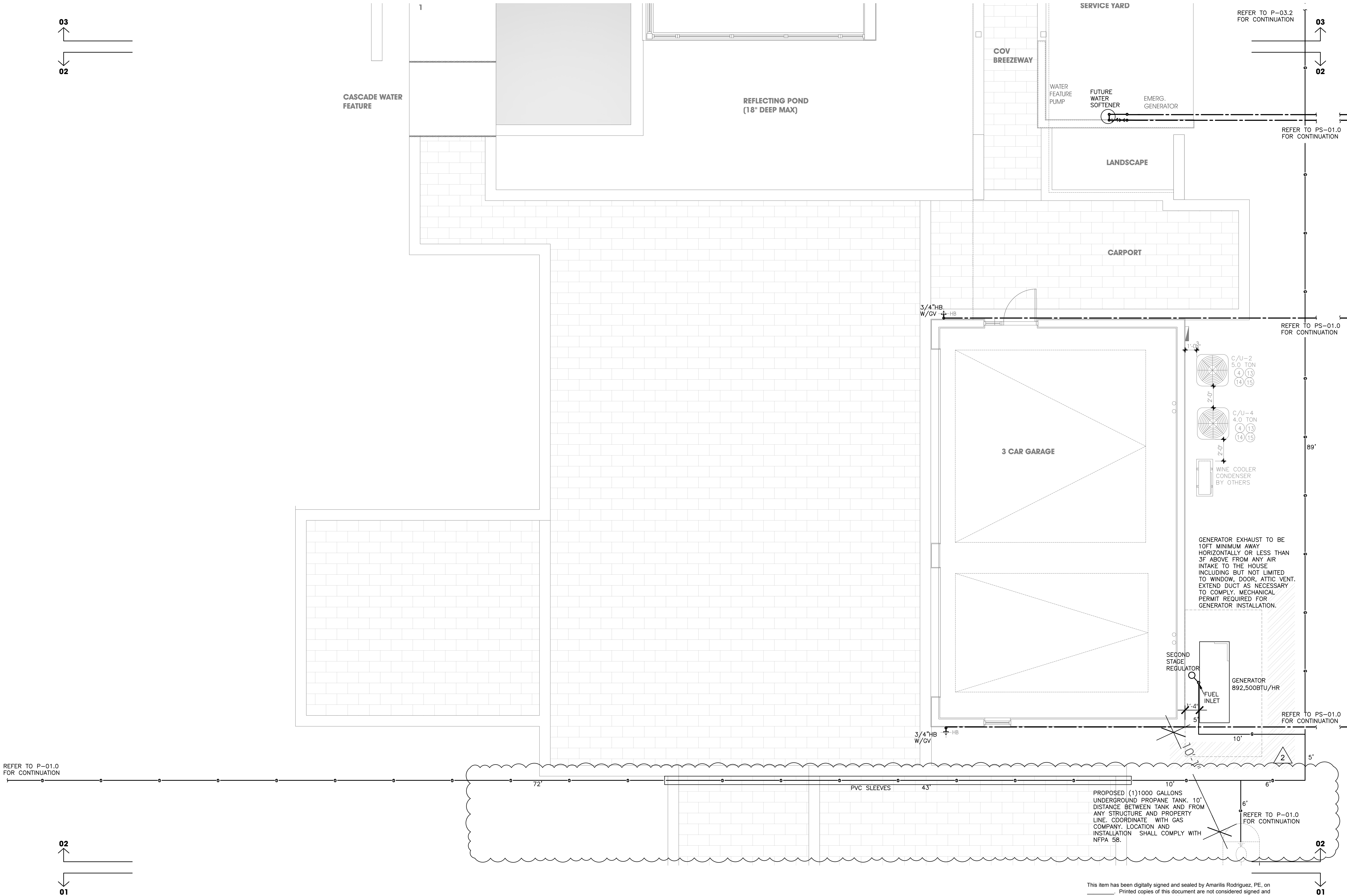
WATER & GAS PARTIAL FIRST FLOOR PLAN: 02 SCALE: 1/4" = 1'-0"
