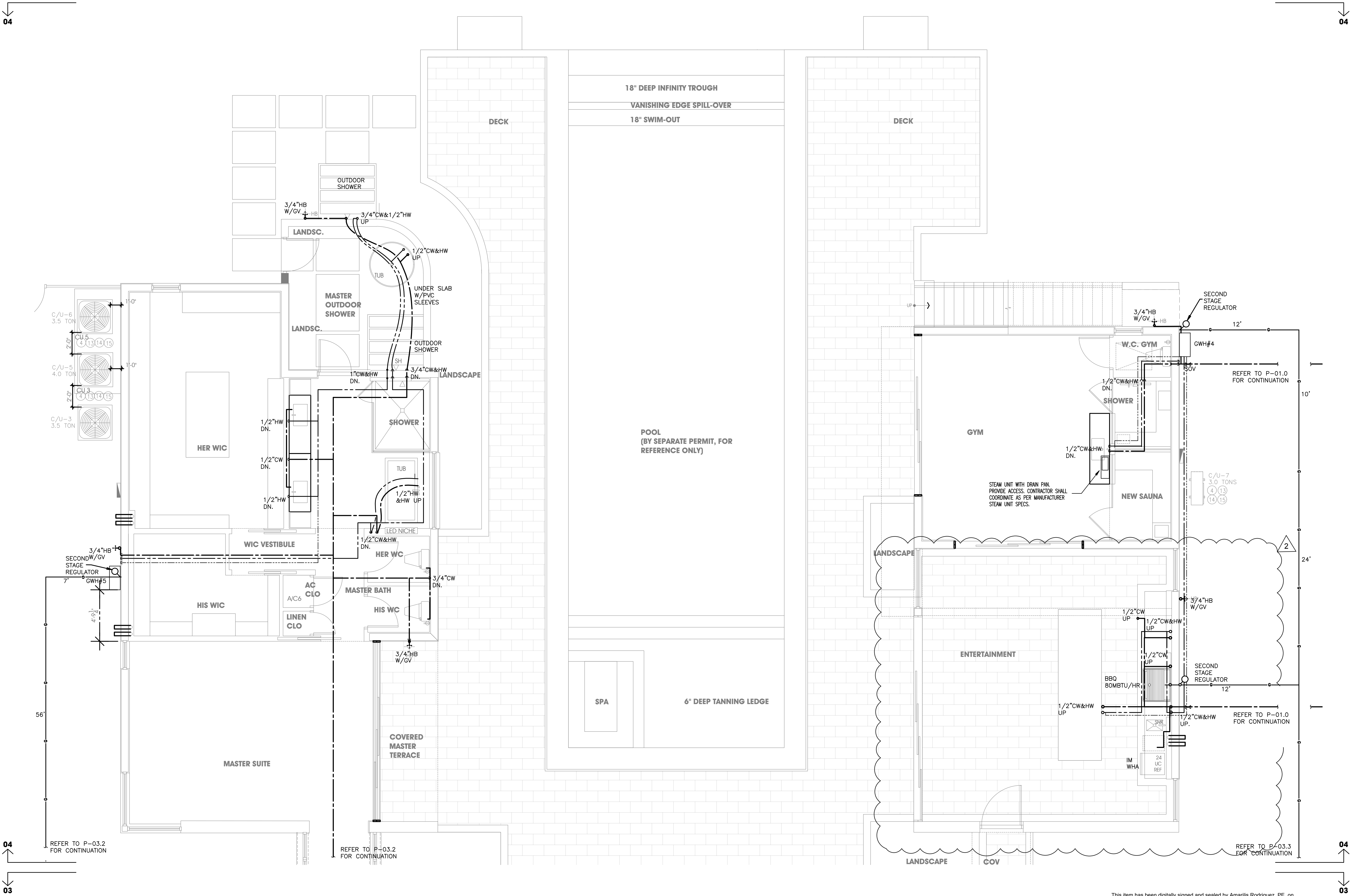
WATER & GAS PARTIAL FIRST FLOOR PLAN: 04 SCALE: 1/4" = 1'-0"
