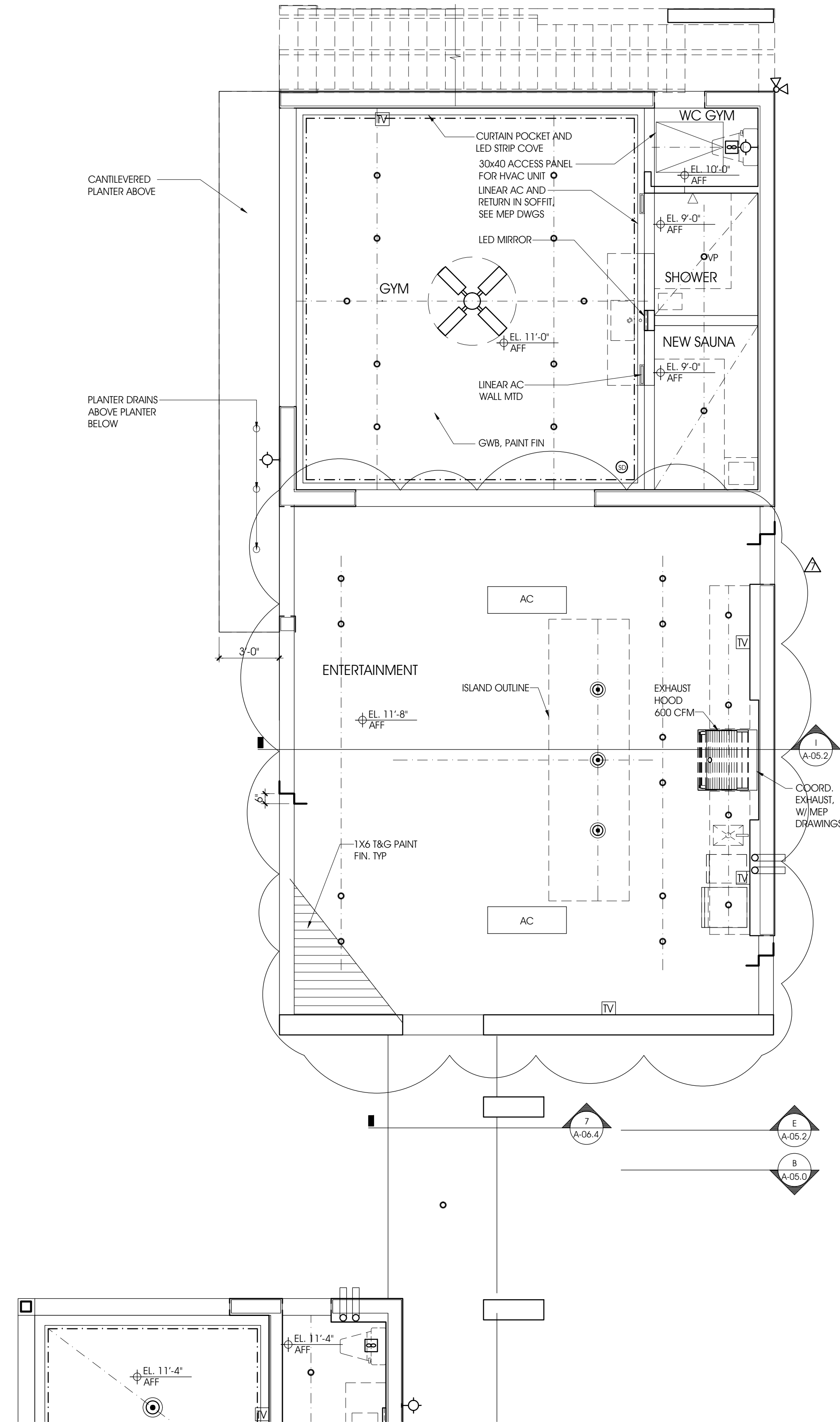
PARTIAL FIRST RCP: 04 SCALE: 1/4" = 1'-0"
