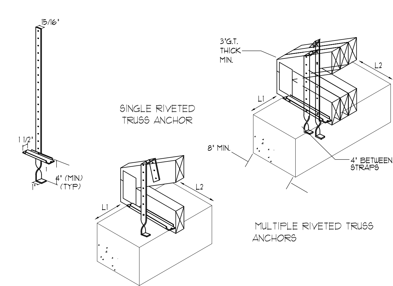
A-X MARK NUMBER OF STRAPS SIZE ASSEMBLY PRODUCT CODE (Nu-Vus) PRODUCT CODE (Nu-Vus) GAUGE DIMENSIONS NUMBER OF 10d COMM NAILS # OF PLY ALLOWABLE LOADS OUT OF CONCRETE OVERHALL LENGTH L-2 L-1 133% 10d COMM. NO.4 A-1 1 16 NVSTA 16 14 16 20 9 1 1430 # 950 # 1426 # 23-0210 #
