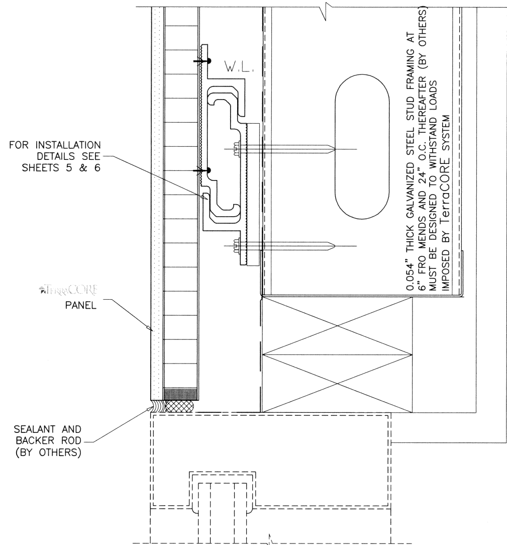
FLUSH WINDOW HEAD
