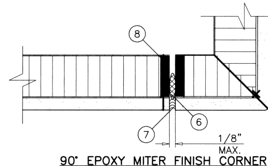
90° EPOXY MITER FINISH CORNER
