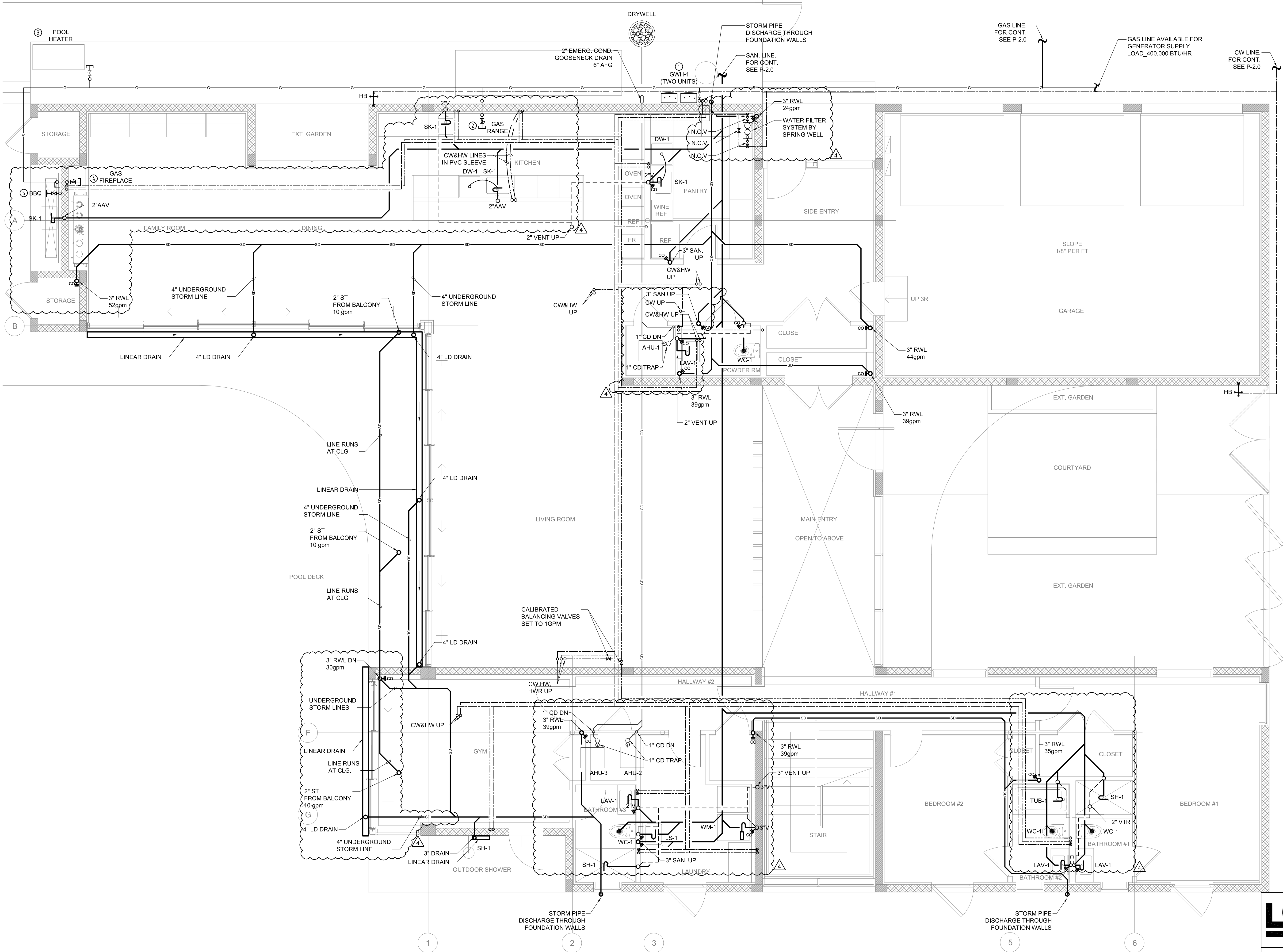
1 PLUMBING - FIRST FLOOR 1/4" = 1'-0"
