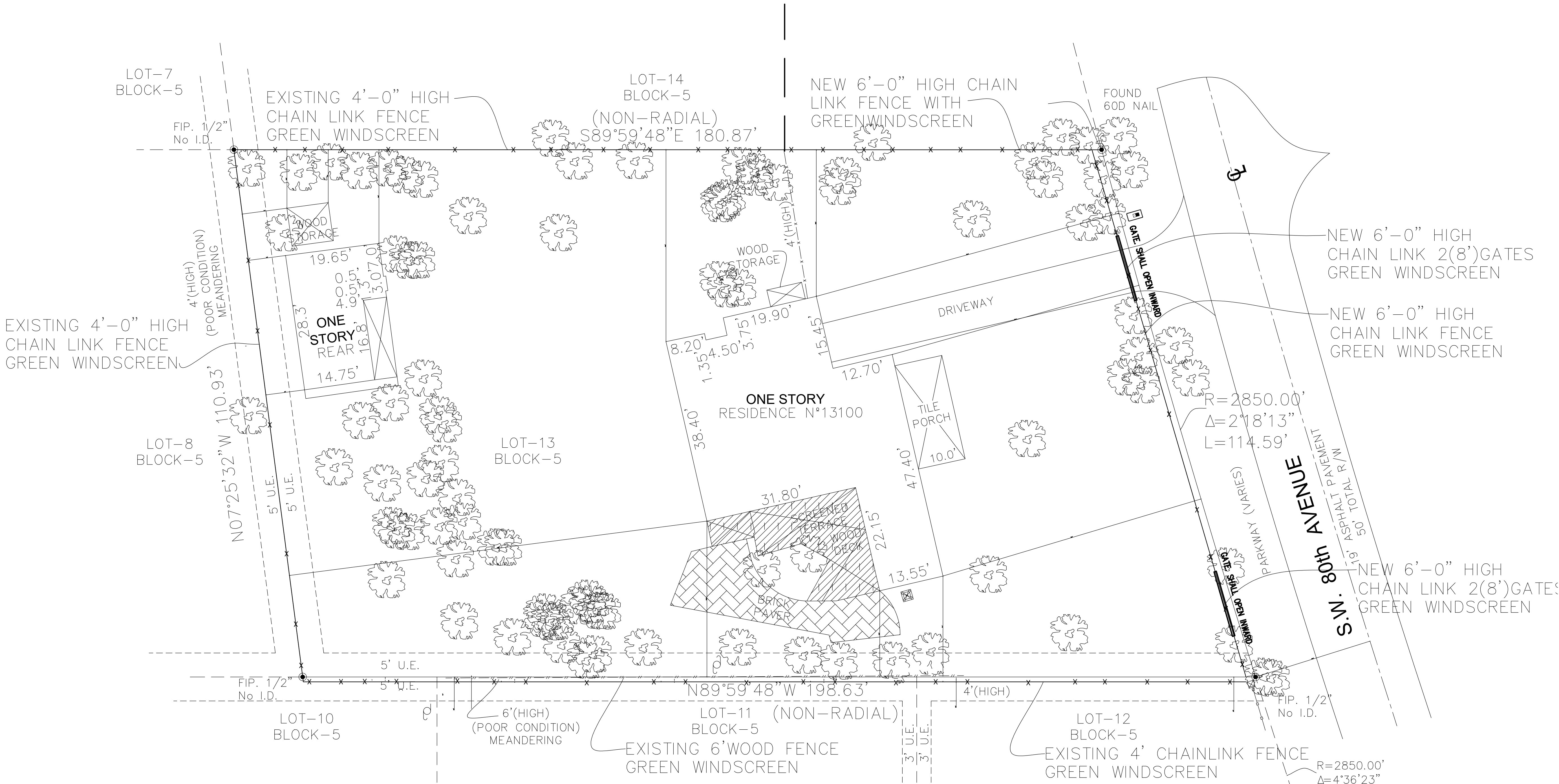
1 TEMP FENCE PLAN 1/8" = 1'-0"
