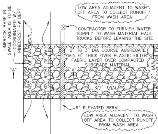
PLAN VIEW
