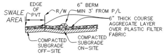
SECTION "A" - "A" FOR EROSION PLAN DETAIL ONLY
