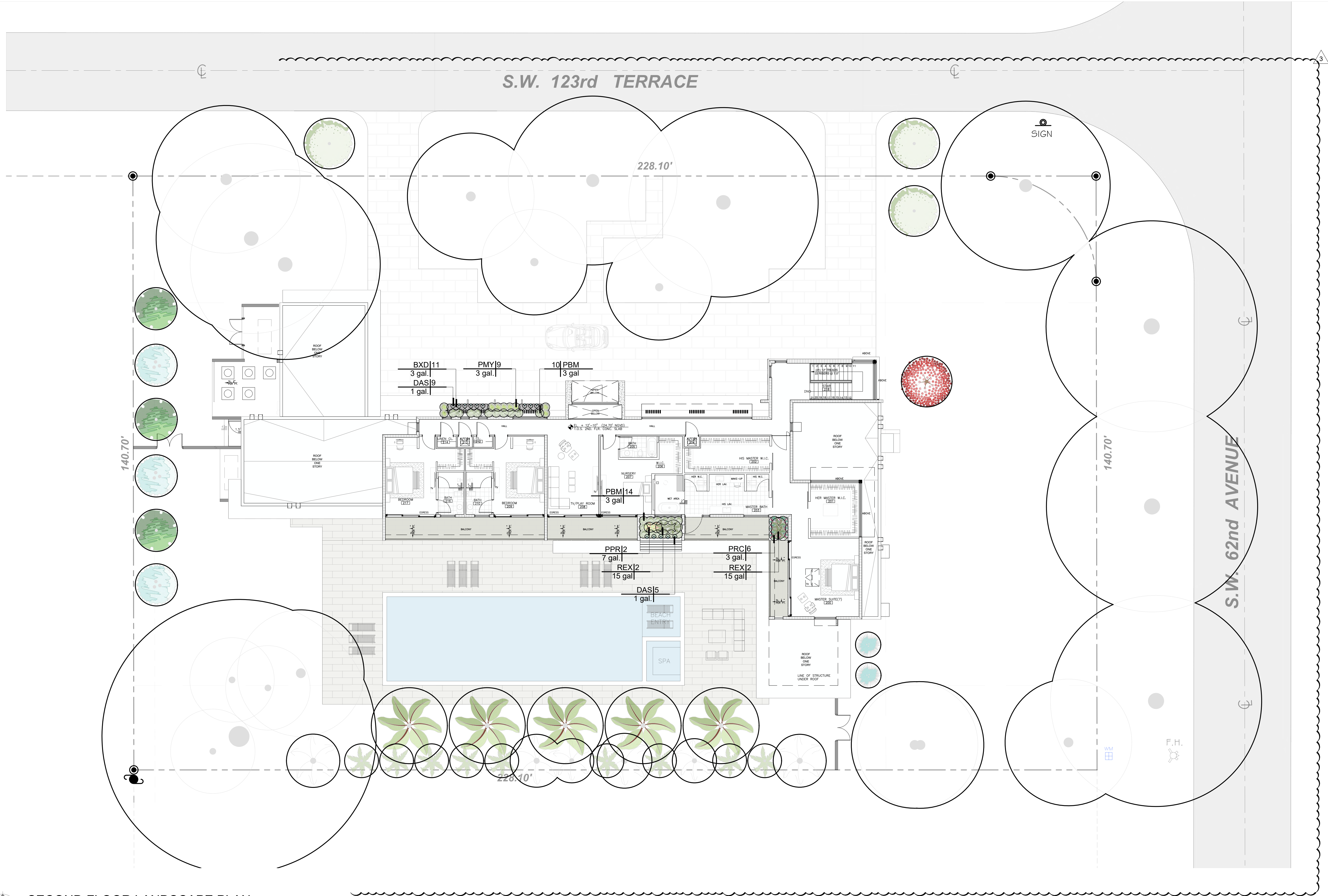
SECOND FLOOR LANDSCAPE PLAN SCALE: 0 10 21 32 feet 3/32" = 1'-0"
