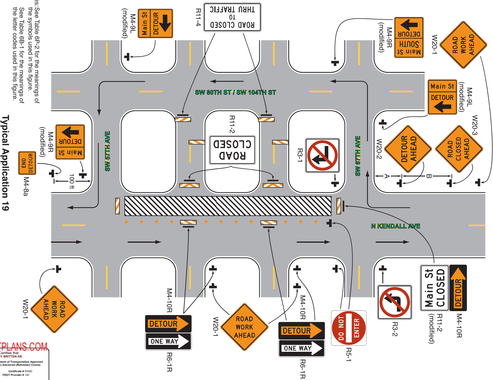
Figure 6P-19. Detour for One Travel Direction (TA-19)
