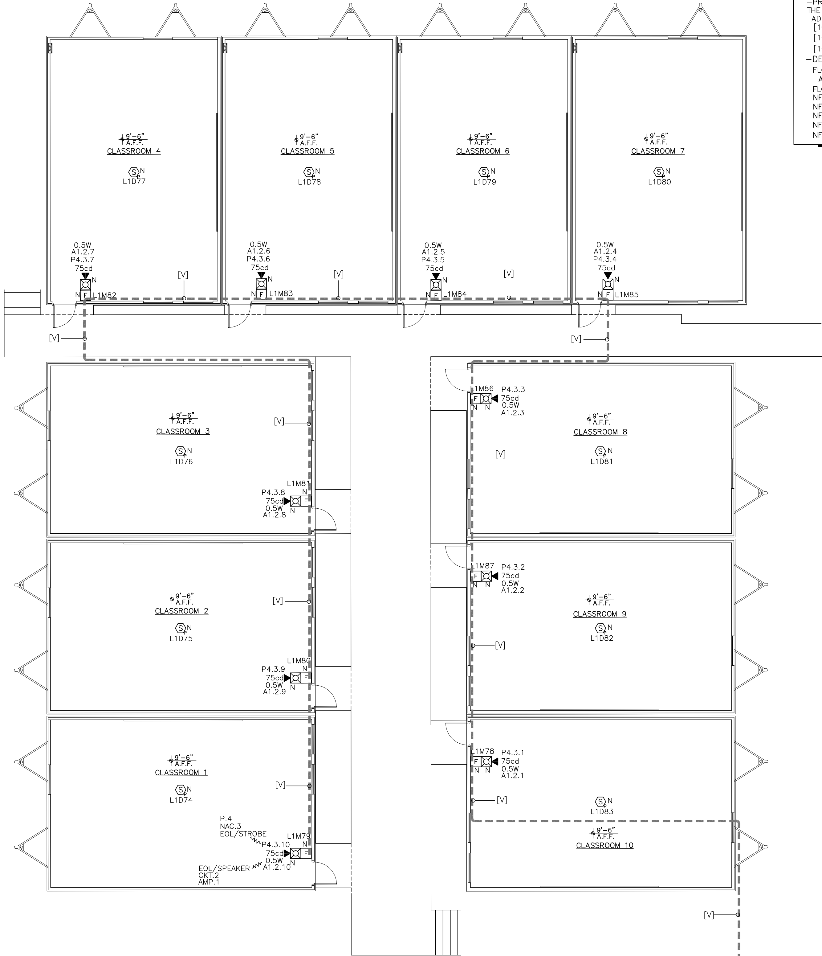
FIRE ALARM FLOOR PLAN PORTABLES [CLASSROOM]
