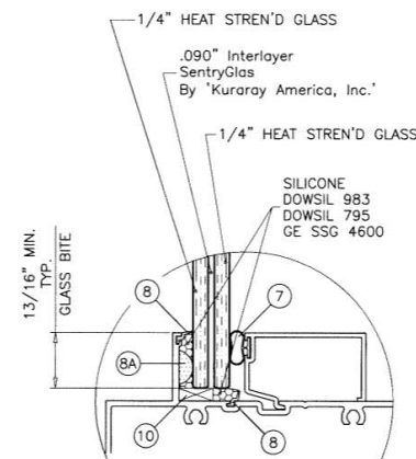
GLASS TYPE 'B'
