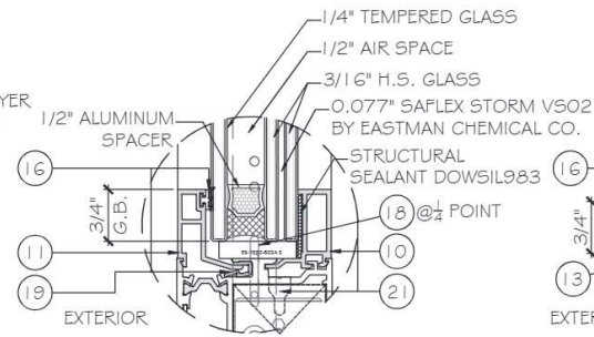
G5 GLASS TYPE 'G5' 1 3/16" NOMINAL OVERALL
