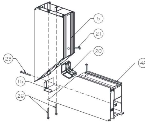
CORNER ASSEMBLY
