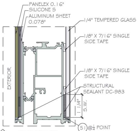
G3 PANEL TYPE 'G3'
