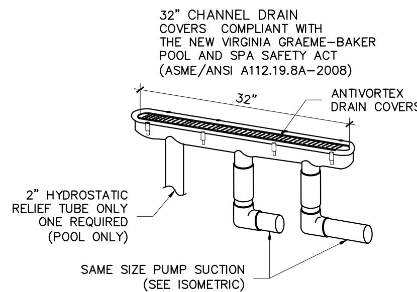
CHANNEL MAINDRAIN DETAIL (SPA) NO SCALE
