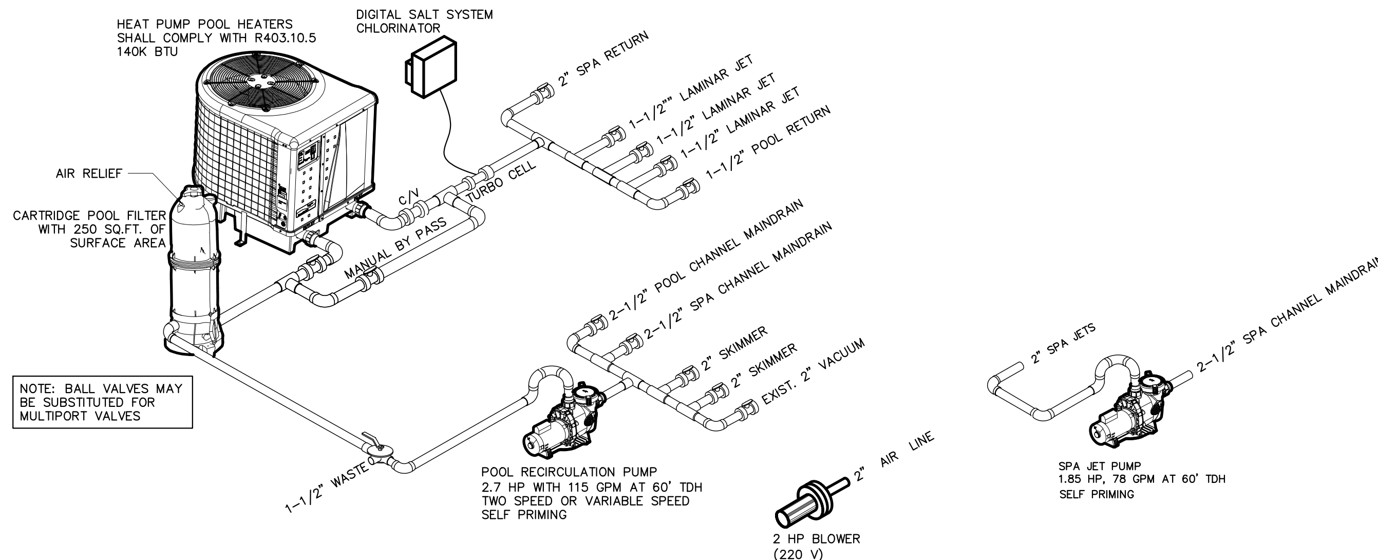
ISOMETRIC
