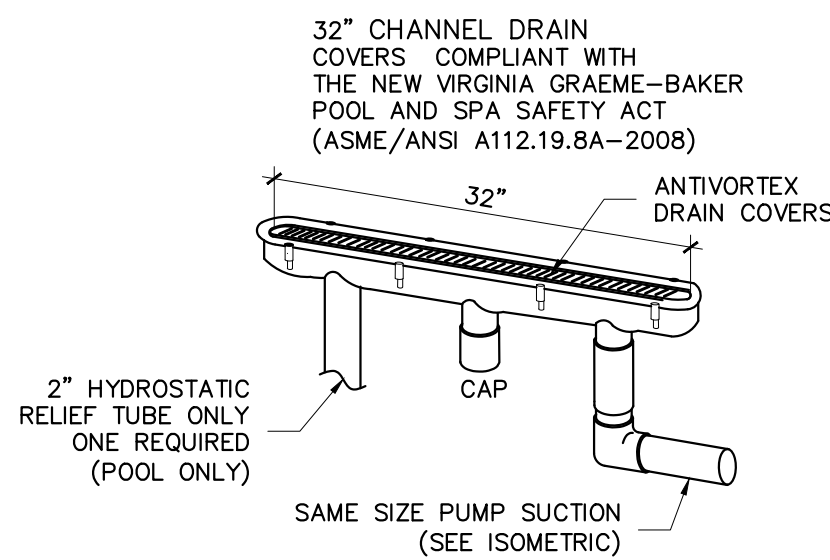
CHANNEL MAINDRAIN DETAIL (POOL) NO SCALE
