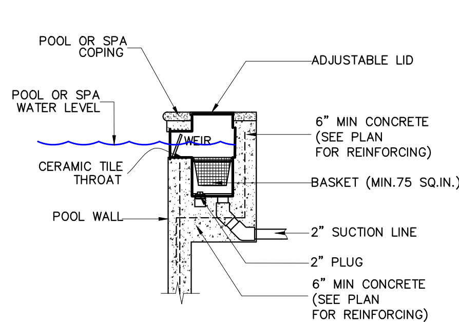
SKIMMER DETAIL NO SCALE
