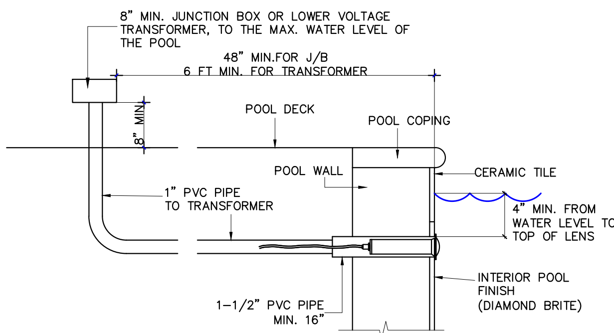
NICHELESS LIGHT DETAIL NO SCALE
