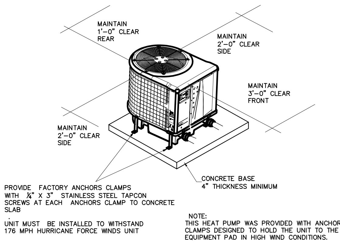
HEAT PUMP MOUNTING DETAIL
