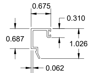
6B GLASS STOP (7/16" GLASS)
