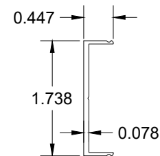
8 JAMB SEAL BASE
