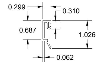
6C GLASS STOP (INSUL. LAM. GLASS)
