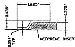
③① ASTRAGAL SEAL (874S)
