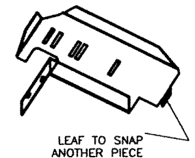
③⑦ EMA BUTTERFLY ANCHOR (PART #PT1-008) FOR DETAILS 2/10, 3/10 4/10 & 6/10 MATERIAL: 18 GA SATIN COAT
