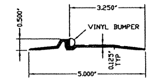
④ THRESHOLD (520S)
