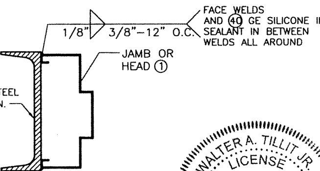
7 INSTALLATION OF JAMB (1) TO STEEL CHANNEL THRU WELDING
