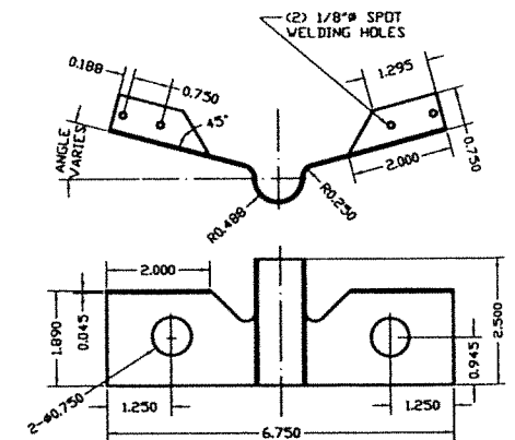
③⑦ EMA BUTTERFLY ANCHOR (PART #PT1-008) FOR DETAILS 2/10, 3/10 4/10 & 6/10 MATERIAL: 18 GA SATIN COAT
