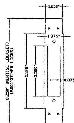
②② FRAME STRIKE REINFORCEMENT
