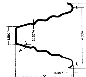
③⑤ WIRE ANCHOR FOR DETAIL #21/17 STEEL WIRE ANCHORS (0.157\"/>
