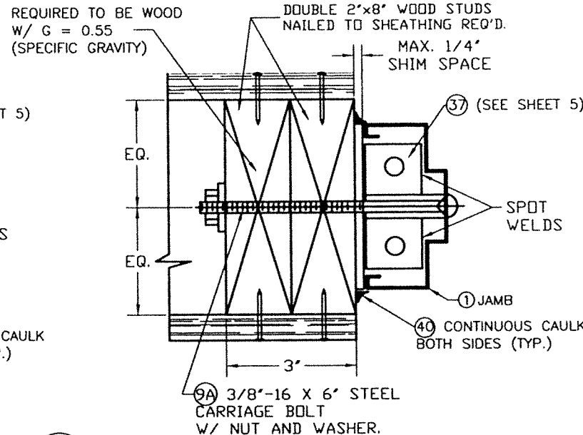
4 INSTALLATION OF 3/8\"/>
