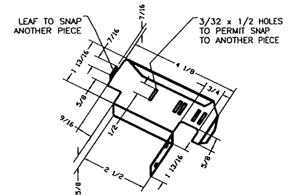
③⑥ 2 PIECE COMBINATION STUD ANCHOR FOR DETAILS #5, 5A/10 CLIPIN STUD ANCHOR MATERIAL: GAUGE 20 (0.035) ASTM A-653, A-60 GALVANNEAL STEEL.
