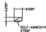
③② PRESS-ON SEAL
