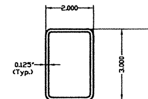
③⑨ REMOVABLE MULLION
