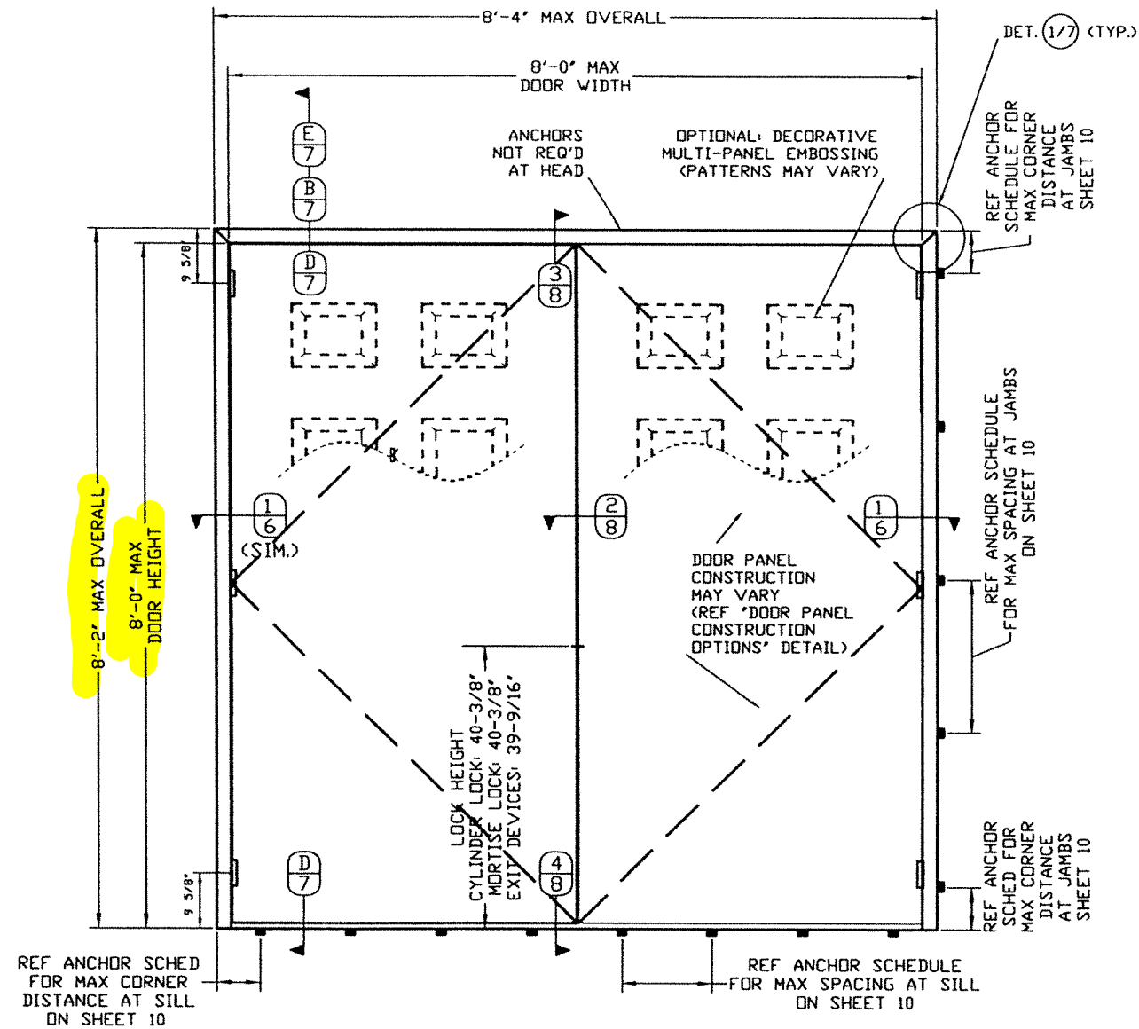
DOUBLE DOOR EXTERIOR ELEVATION: SERIES 8080
