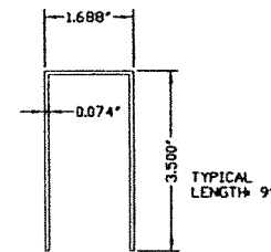
②⑤ SURFACE BOLT REINFORCEMENT
