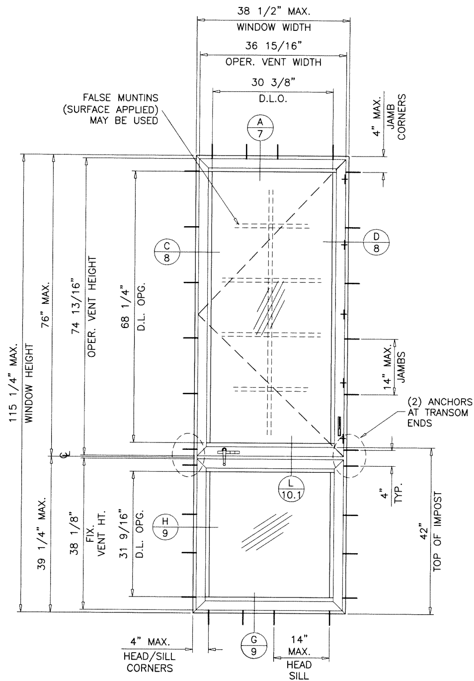
TYPICAL ELEVATIONS
