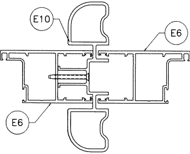
REINF. ASTRAGAL
