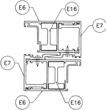
REINF. INTERLOCK
