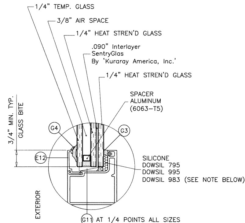
GLASS TYPE 'AI' 1-3/16" OVERALL INSUL. LAM. GLASS
