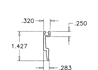
E9.1 GLASS STOP (INSUL. LAM. GLASS)
