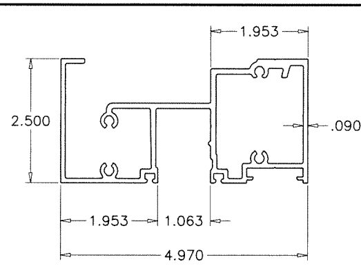
T1 TRANSOM HEADER Series 9500
