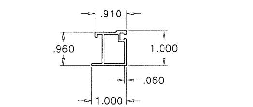
T3 TRANSOM GLASS STOP
