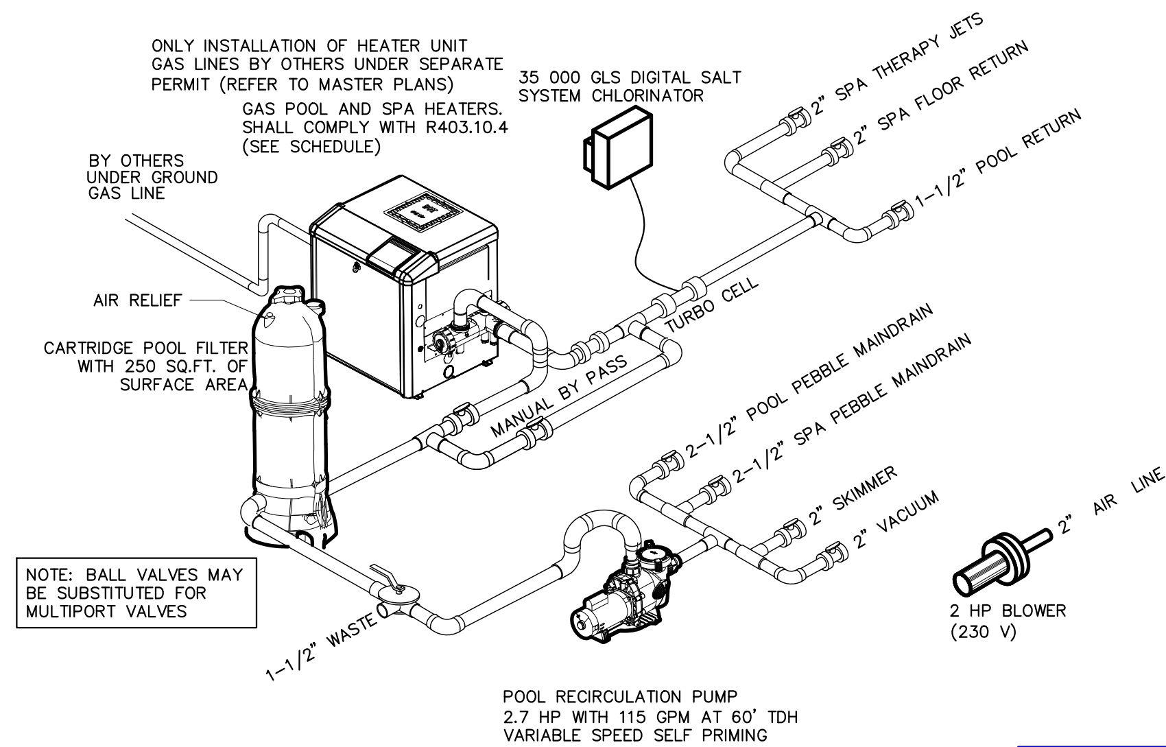
ISOMETRIC
