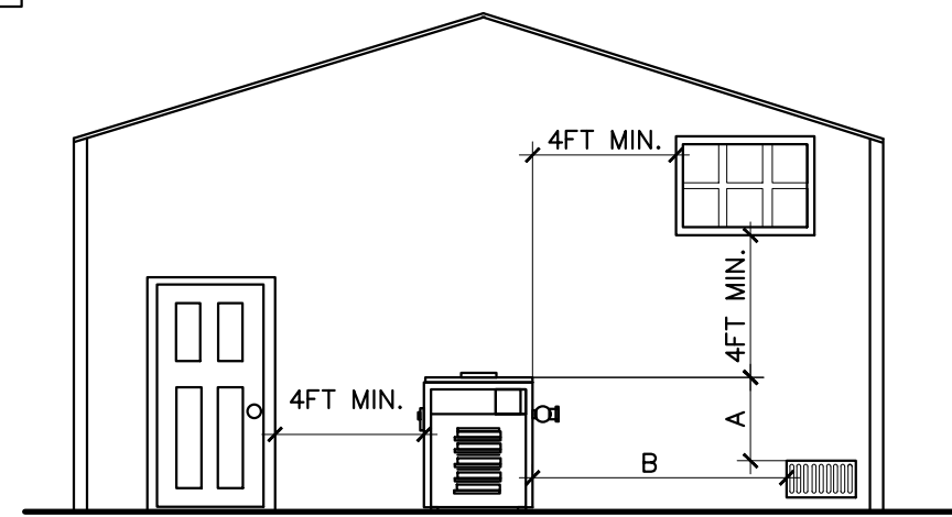
OUTDOOR HEATER INSTALLATION
