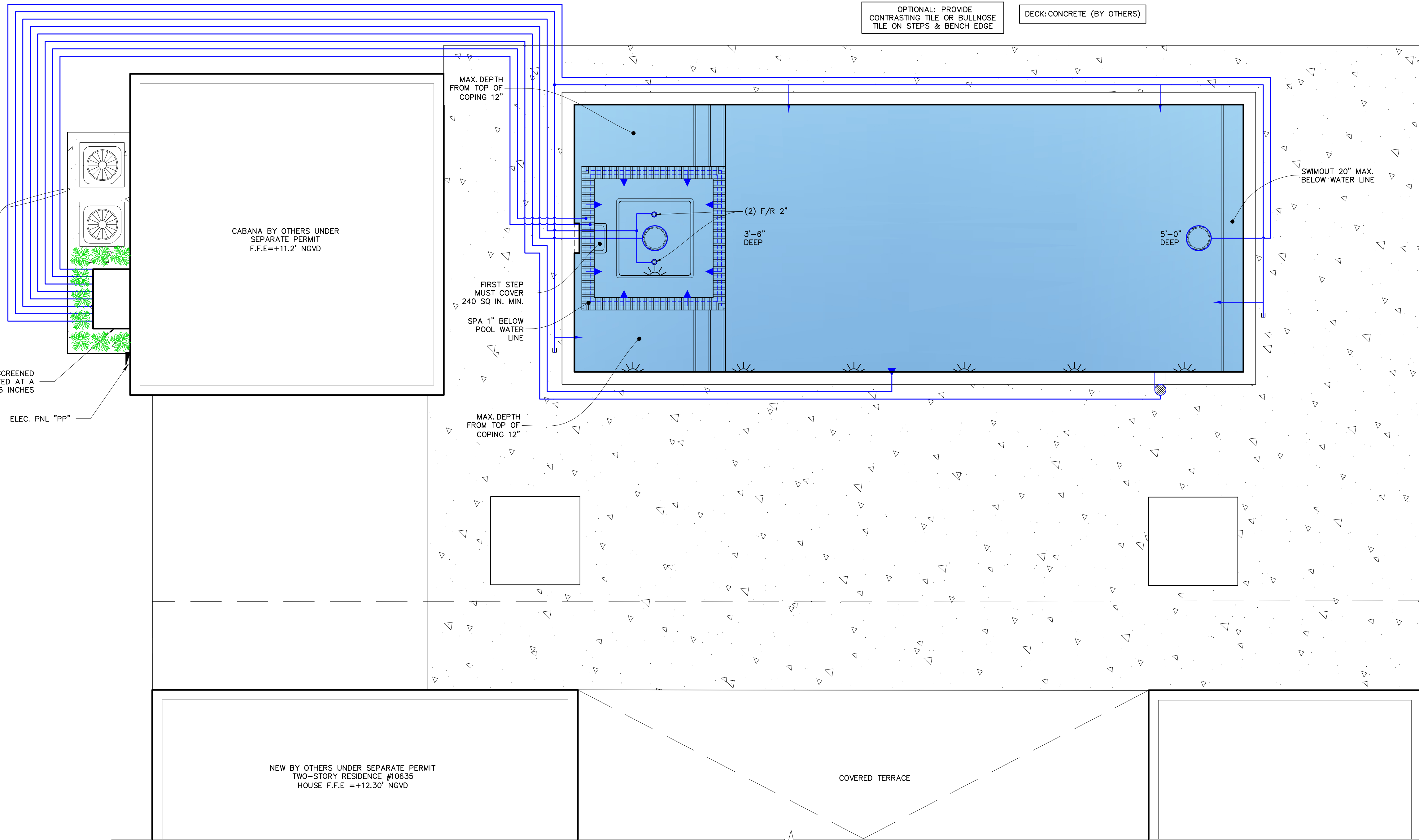
POOL PLUMBING PLAN SCALE: 1/4"=1'-0"
