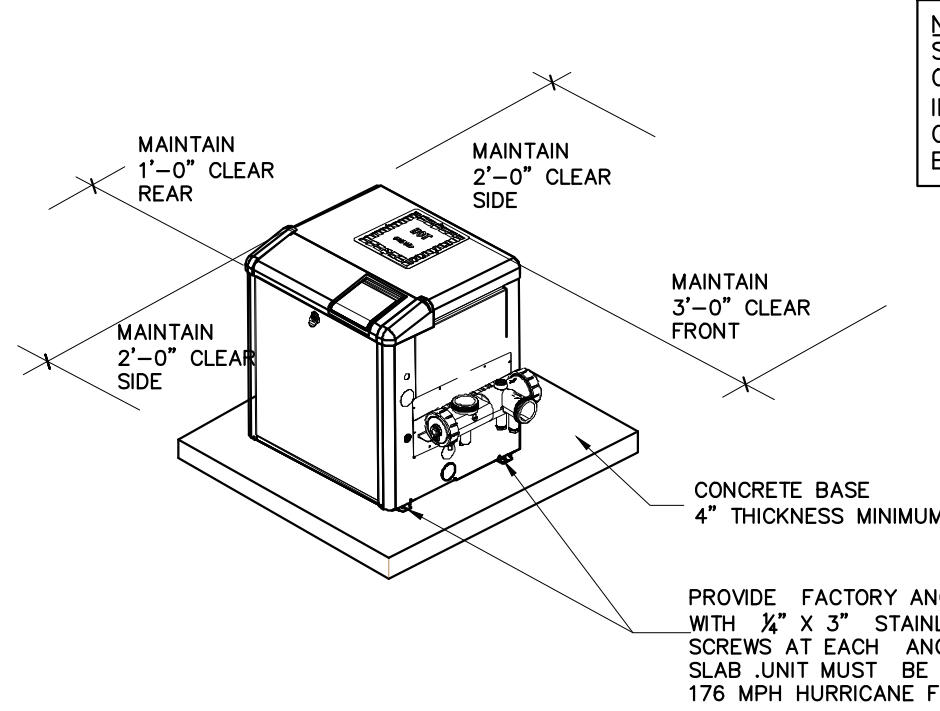
GAS HEATER MOUNTING DETAIL NO SCALE
