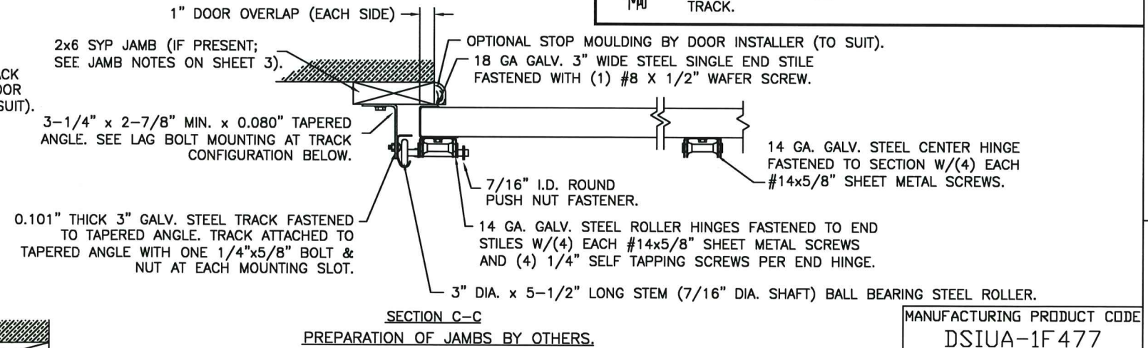
JAMB CONFIGURATION DOORS 800 LBS AND OVER.
