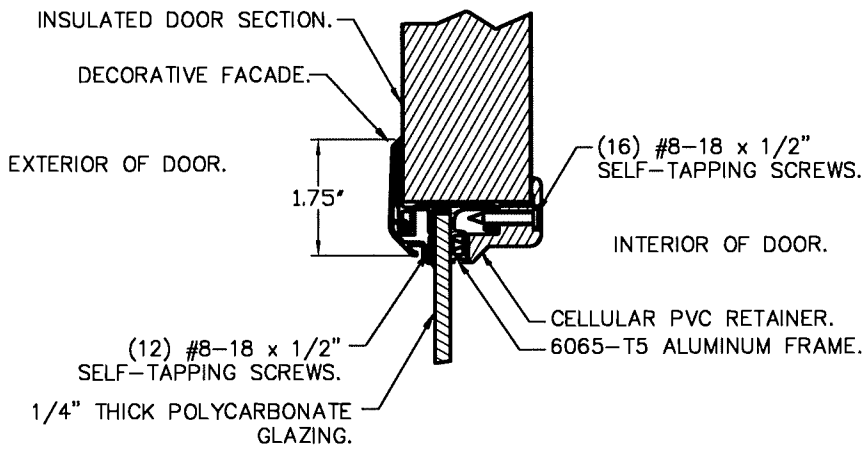
IMPACT-RESISTANT ASSEMBLY DETAILS
