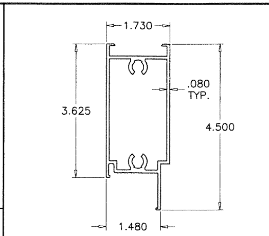
E4 TOP AND BOTTOM RAIL
