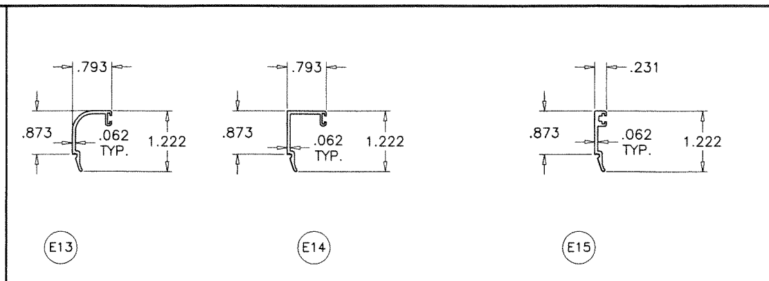
E13 GLASS STOP (LAM. GLASS)
