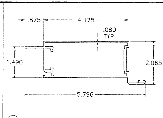
E9 ASTRAGAL STILE (ACTIVE)
