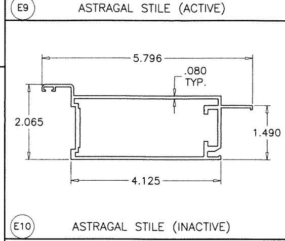
E9 ASTRAGAL STILE (ACTIVE)
