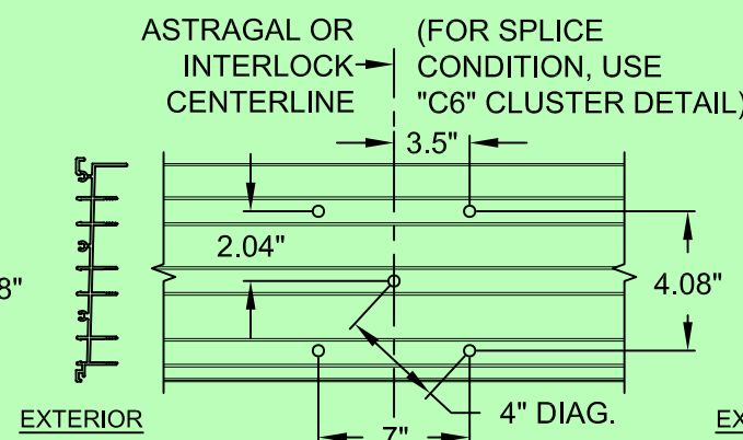
3-TRACK FRAME HEAD/SILL @ ASTRAGAL OR INTERLOCK (USE WHERE 5 CLUSTER ANCHORS ARE REQUIRED, "C5")
