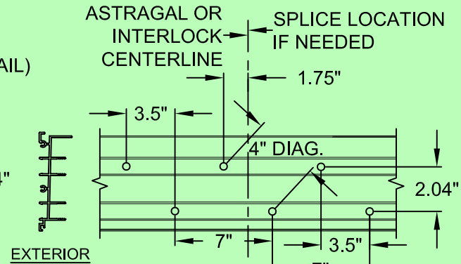
2-TRACK FRAME HEAD/SILL @ ASTRAGAL OR INTERLOCK (USE WHERE 6 CLUSTER ANCHORS ARE REQUIRED, "C6")
