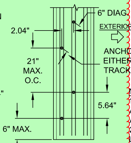
3-TRACK FRAME JAMB ANCHOR PAIR
