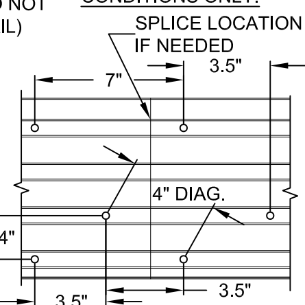
4-TRACK FRAME HEAD/SILL @ ASTRAGAL OR INTERLOCK (USE WHERE 6 CLUSTER ANCHORS ARE REQUIRED, "C6") WITH & WITHOUT SPLICE CONDITION
