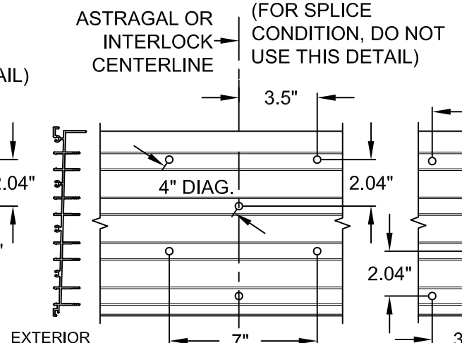
4-TRACK FRAME HEAD/SILL @ ASTRAGAL OR INTERLOCK (USE WHERE 6 CLUSTER ANCHORS ARE REQUIRED, "C6") WITH & WITHOUT SPLICE CONDITION
