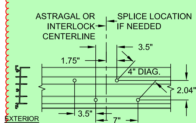
2-TRACK FRAME HEAD/SILL @ ASTRAGAL OR INTERLOCK (USE WHERE 4 CLUSTER ANCHORS ARE REQUIRED, "C4")
