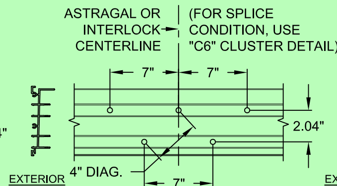
2-TRACK FRAME HEAD/SILL @ ASTRAGAL OR INTERLOCK (USE WHERE 5 CLUSTER ANCHORS ARE REQUIRED, "C5")
