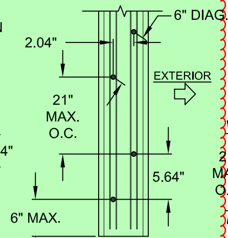
2-TRACK FRAME JAMB ANCHOR PAIR
