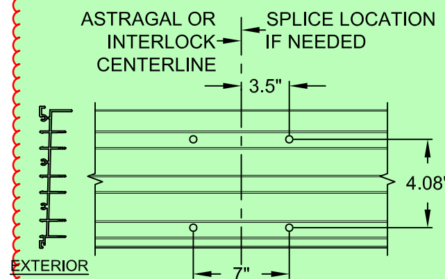
3-TRACK FRAME HEAD/SILL @ ASTRAGAL OR INTERLOCK (USE WHERE 4 CLUSTER ANCHORS ARE REQUIRED, "C4")
