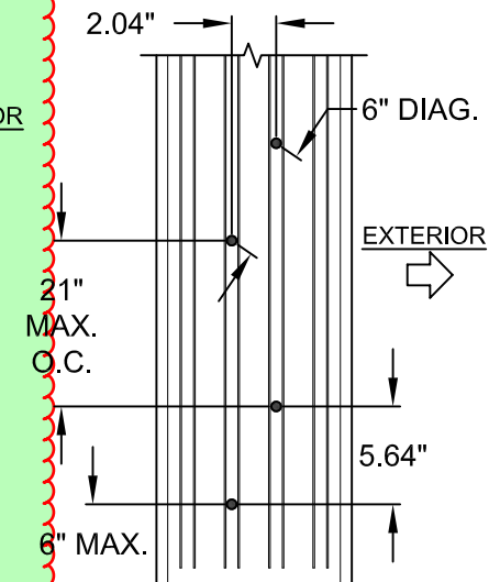
4-TRACK FRAME JAMB ANCHOR PAIR
