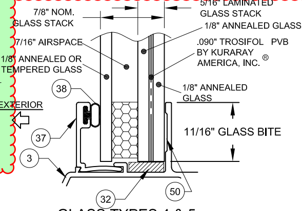
GLASS TYPES 4 & 5
