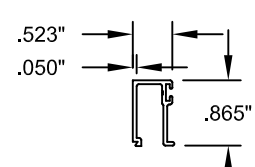
36 BEAD C #7042, 6063-T6
