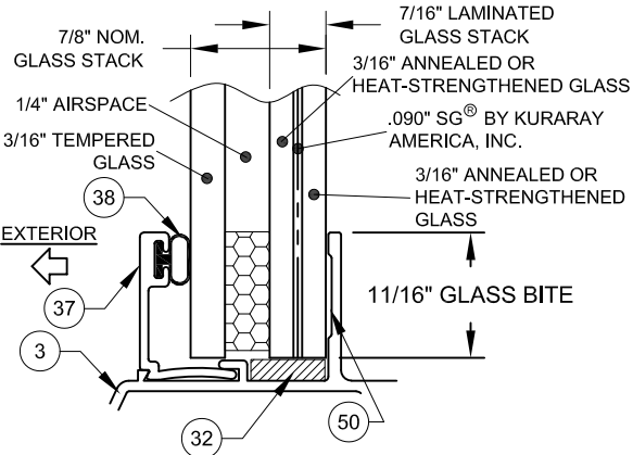
GLASS TYPES 8 & 9
