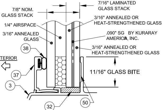
GLASS TYPES 6 & 7
