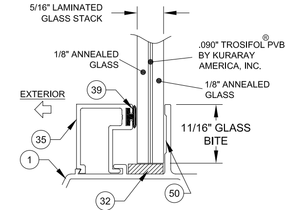
GLASS TYPE 1
