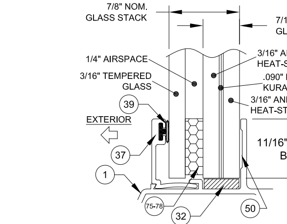
GLASS TYPES 4 & 5
