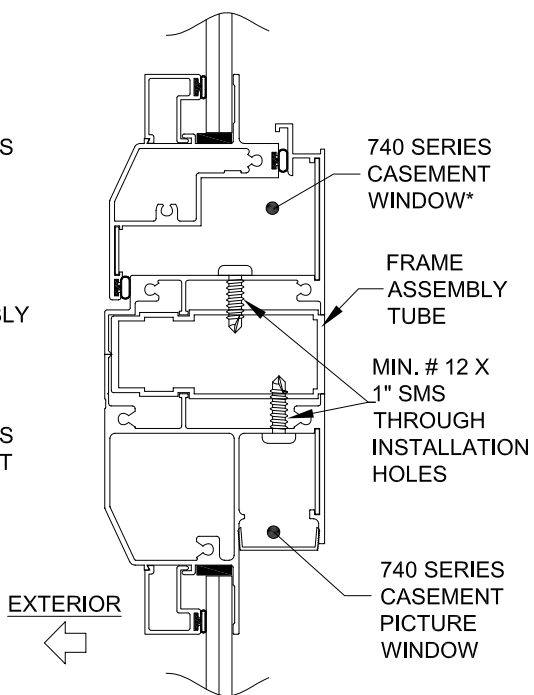
VERTICAL SECTION E-E
