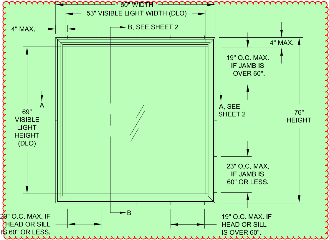
TYP. ELEVATION OF CASEMENT PICTURE WINDOW
