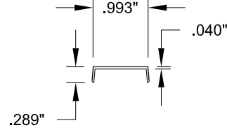
3 INST. HOLE COVER #7007, 6063-T6
