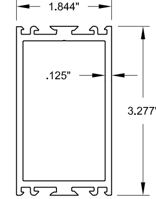
8 HORIZONTAL MUNTIN
