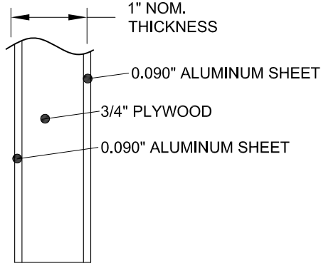
COMPOSITE TYPE 10 ALUM., OPAQUE, COMPOSITE PANEL
