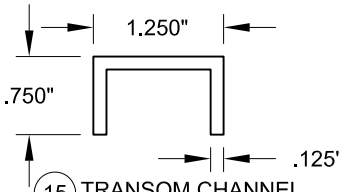
15 TRANSOM CHANNEL
