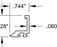
22 I.G. STOP
