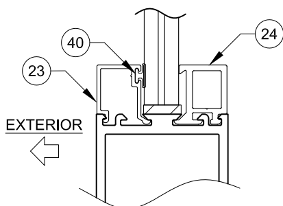
LAMI. GLAZING DETAIL SHOWN WITH OPT. SQUARE BEADING.
