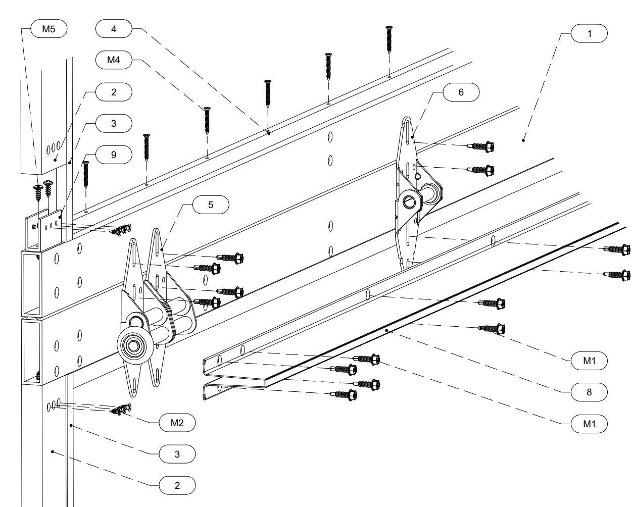
INSTALLATION DETAIL
