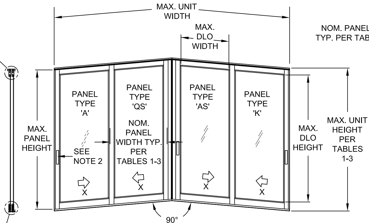
EXAMPLE: 90° INSIDE CORNER, 4 PANELS - XX/XX
