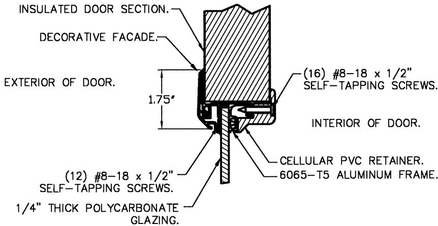
IMPACT-RESISTANT ASSEMBLY DETAILS
