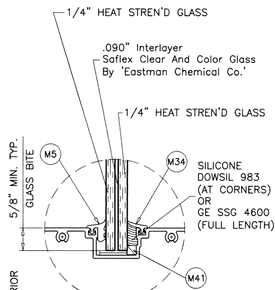
GLASS TYPE 'A' 9/16" OVERALL LAM. GLASS
