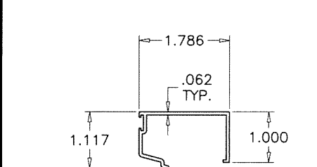
E33 TRANSOM GLASS STOP (ES-8000)
