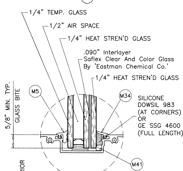
GLASS TYPE 'Ci' 1-5/16" OVERALL INSUL. LAM. GLASS
