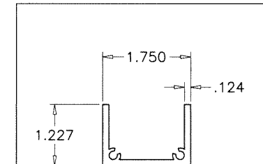
E56 SUPPORT GUIDE
