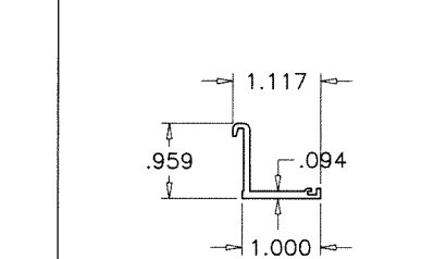
E36 TRANSOM GLAZING ADAPTER
