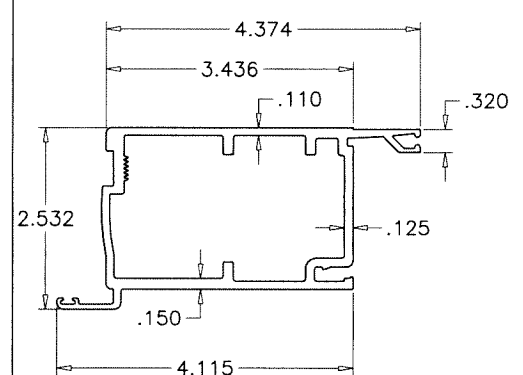
E8A ALT. MEETING STILE - ACTIVE LEAF
