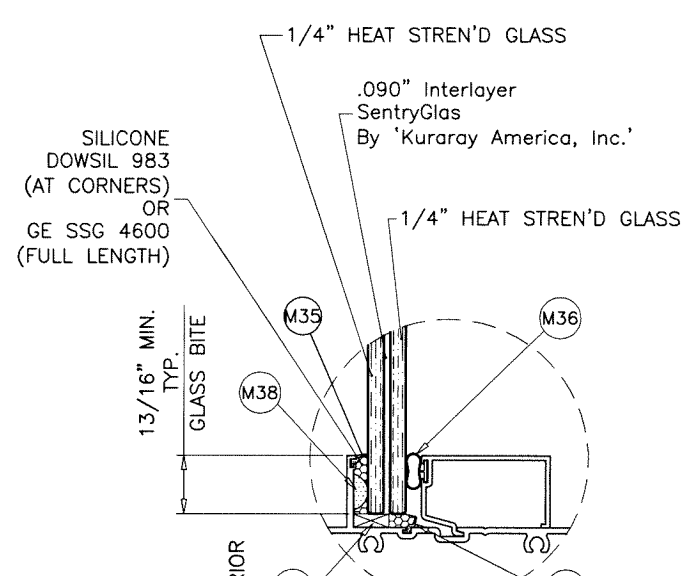
GLASS TYPE 'B' 9/16" OVERALL LAM. GLASS
