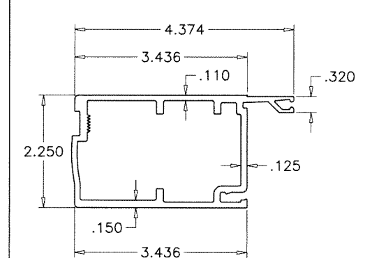
E8 MEETING STILE - ACTIVE LEAF
