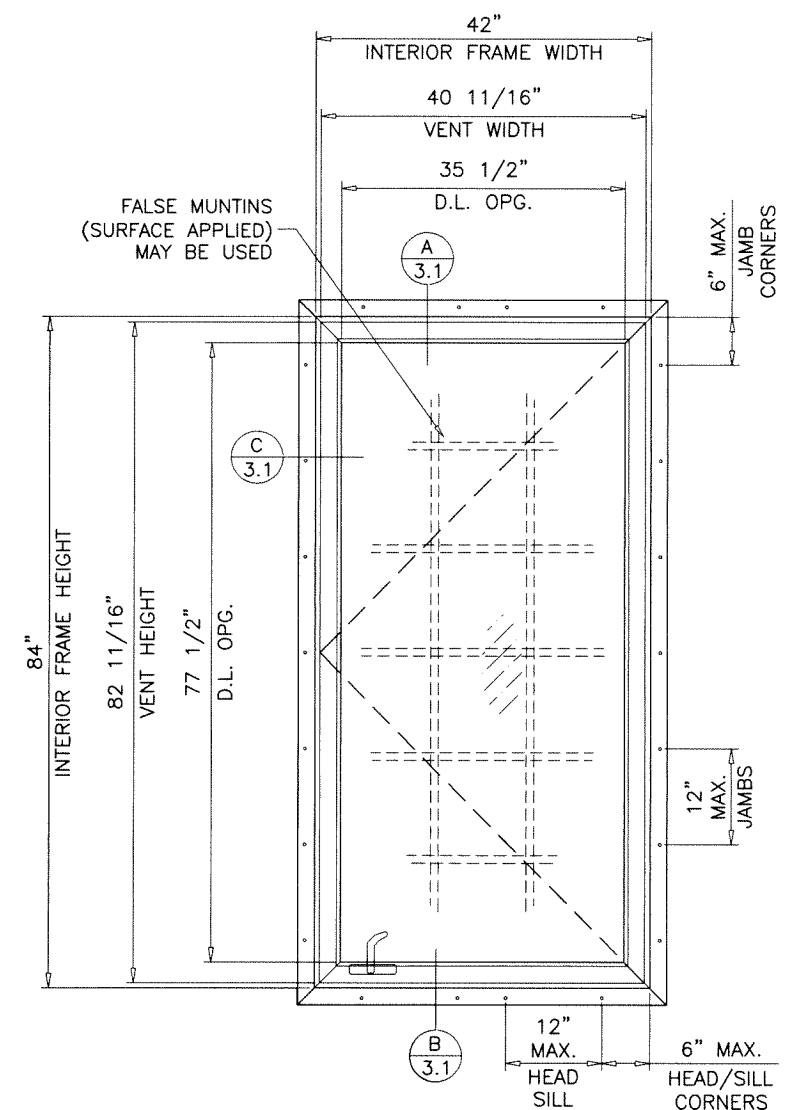
TYPICAL ELEVATION ANCHORS THRU NAIL FIN
