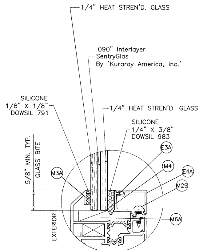
GLASS TYPE 'B1' 9/16" OVERALL NOM. THK.
