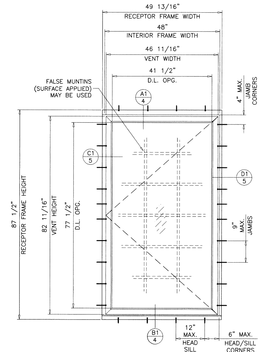
TYPICAL ELEVATION ANCHORS THRU RECEPTOR FRAMES
