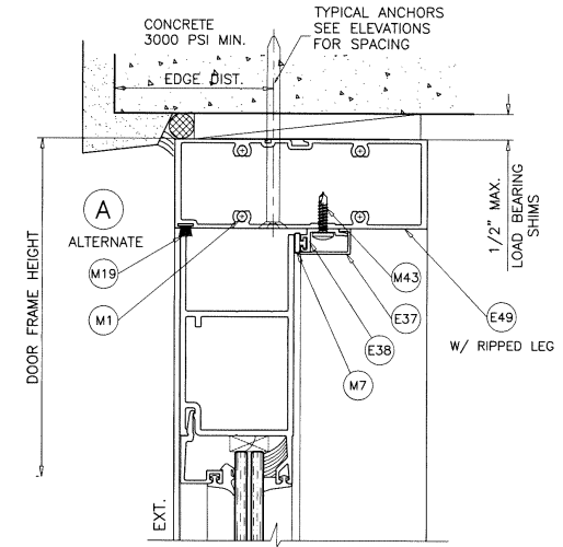
DOOR HEAD SERIES-8000 FRAME OPTION
