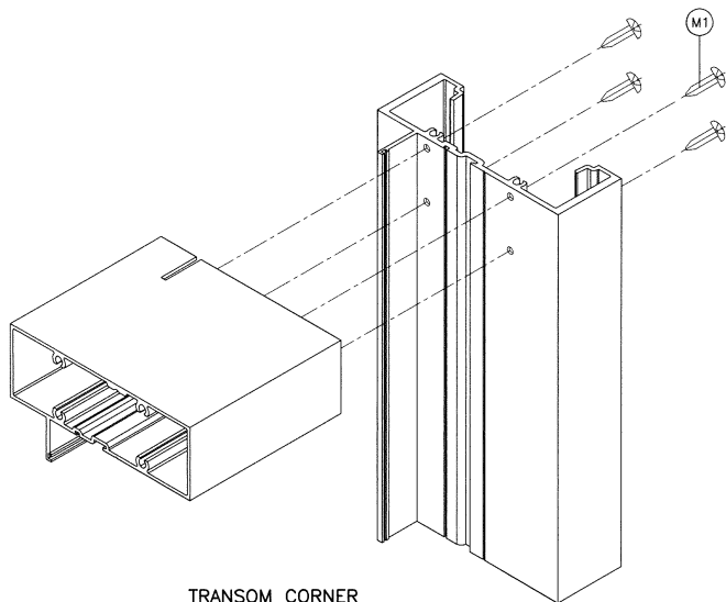
TRANSOM CORNER SERIES-8000 WINDOW WALL
