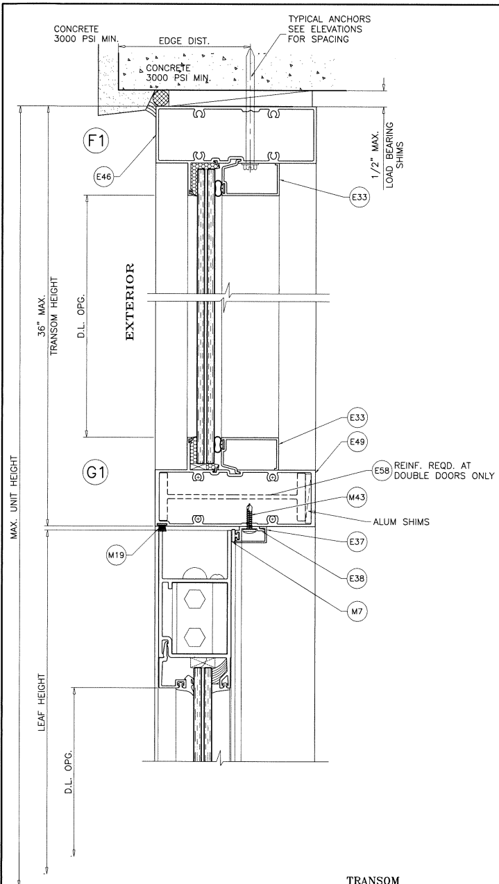
TRANSOM SERIES-8000 FRAMES OPTION
