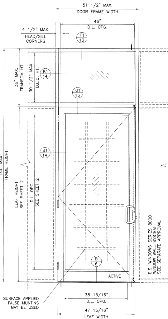
TYPICAL ELEVATION SINGLE (O/X) STD. THRESHOLD (ES-8000 TRANSOM)
