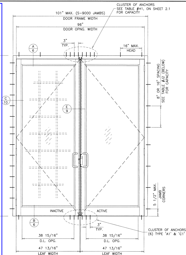
TYPICAL ELEVATION DOUBLE (XX) STD. THRESHOLD
