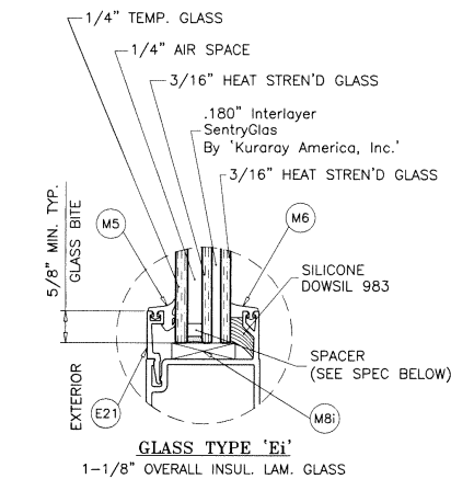
GLAZING OPTIONS (LEVEL 'E' IMPACT) DOOR LEAF
