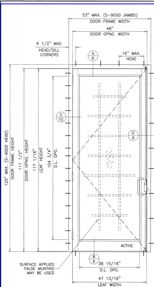
TYPICAL ELEVATION SINGLE (X) STD. THRESHOLD
