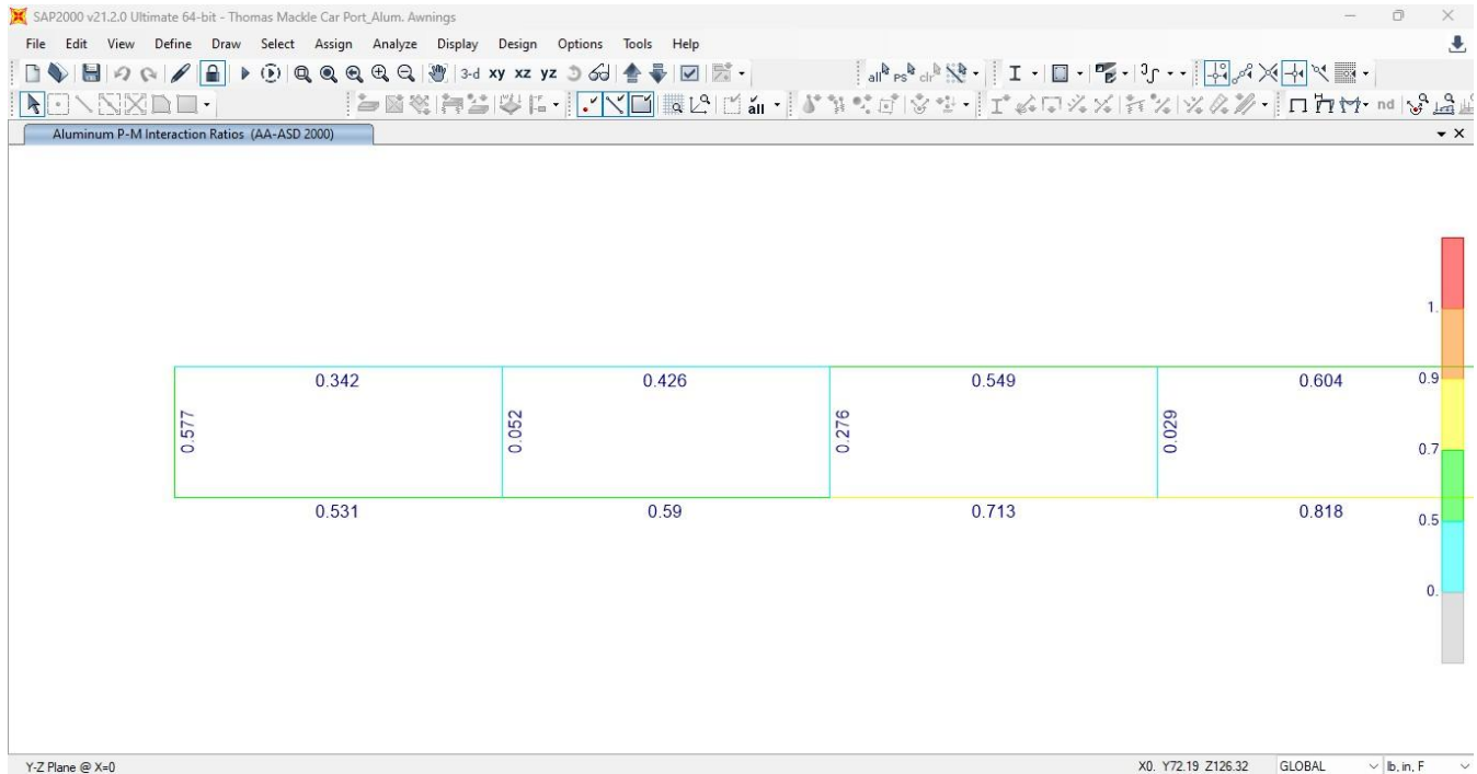
P-M RATIO COLORS AND VALUES – ELEVATION VIEW OF SIDE FLAT BEAM H=12" (ALL MEMBERS PASS)
