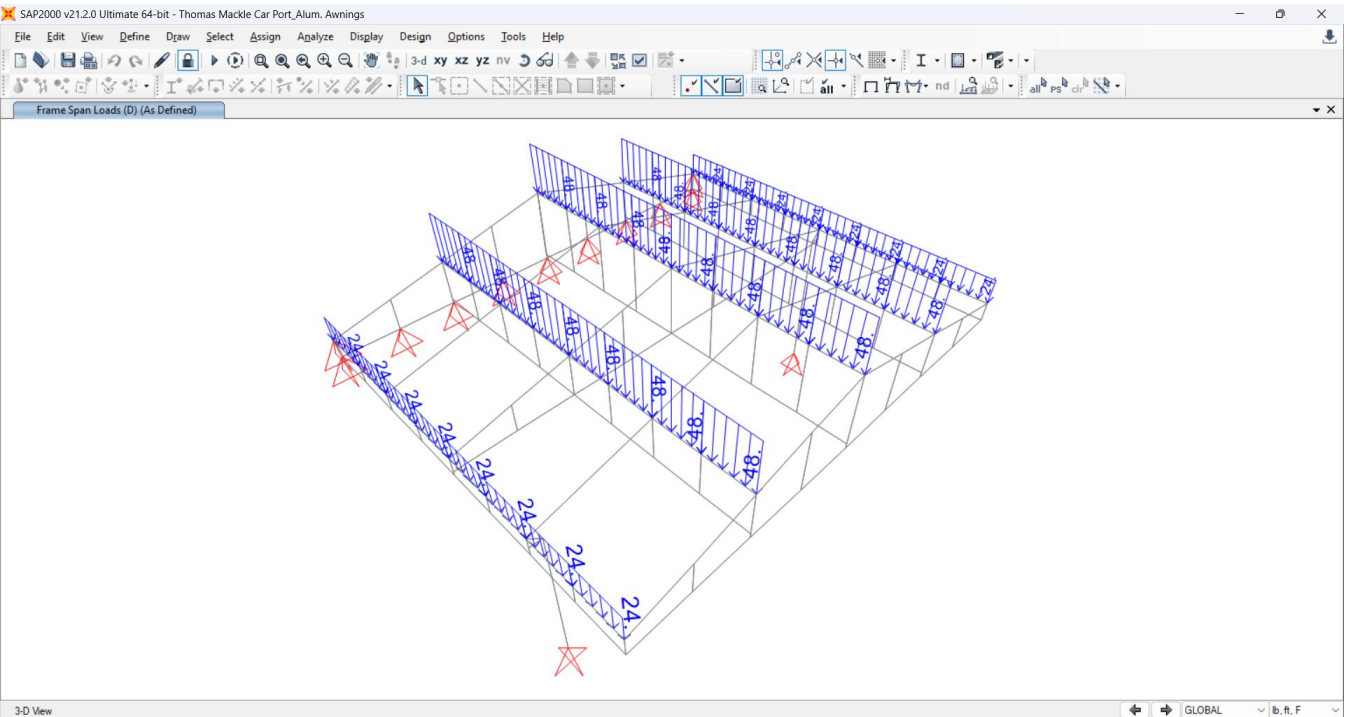
3D VIEW - DEAD LOADS APPLIED (Lb/ft)
