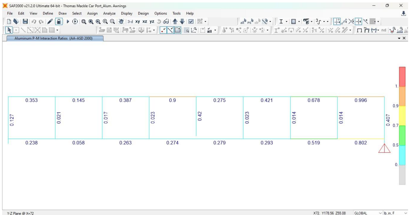
P-M RATIO COLORS AND VALUES – ELEVATION VIEW OF MIDDLE FLAT BEAM H=27" (ALL MEMBERS PASS)
