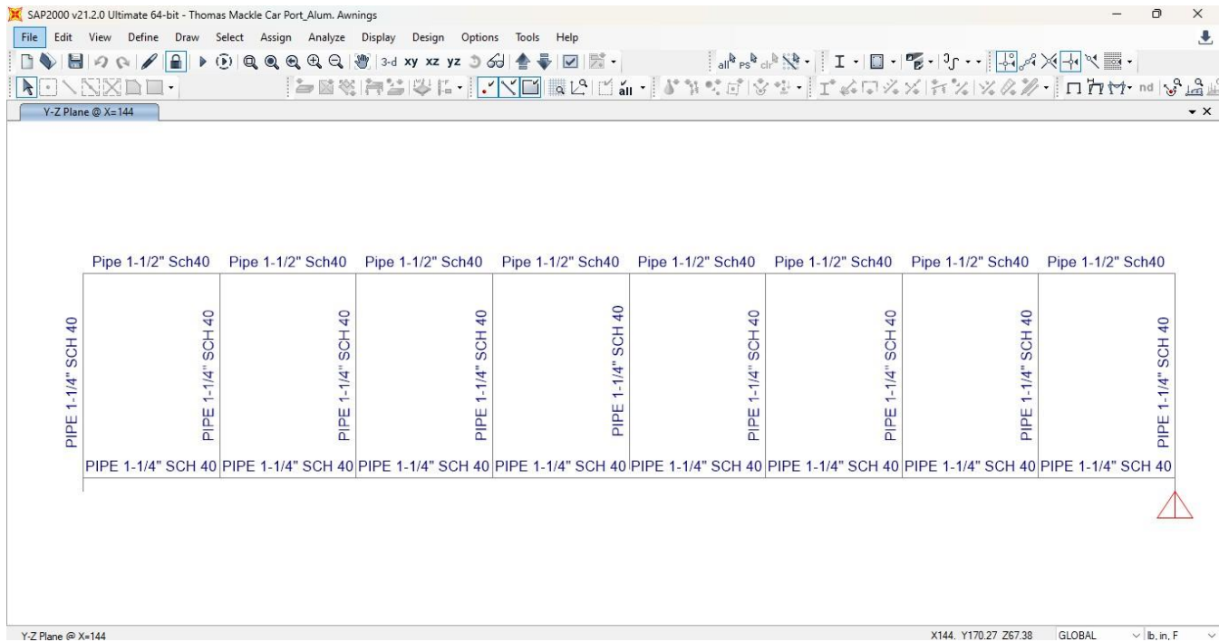
ELEVATION VIEW OF PRINCIPAL FLAT BEAM H=45" _DESIGN SECTIONS
