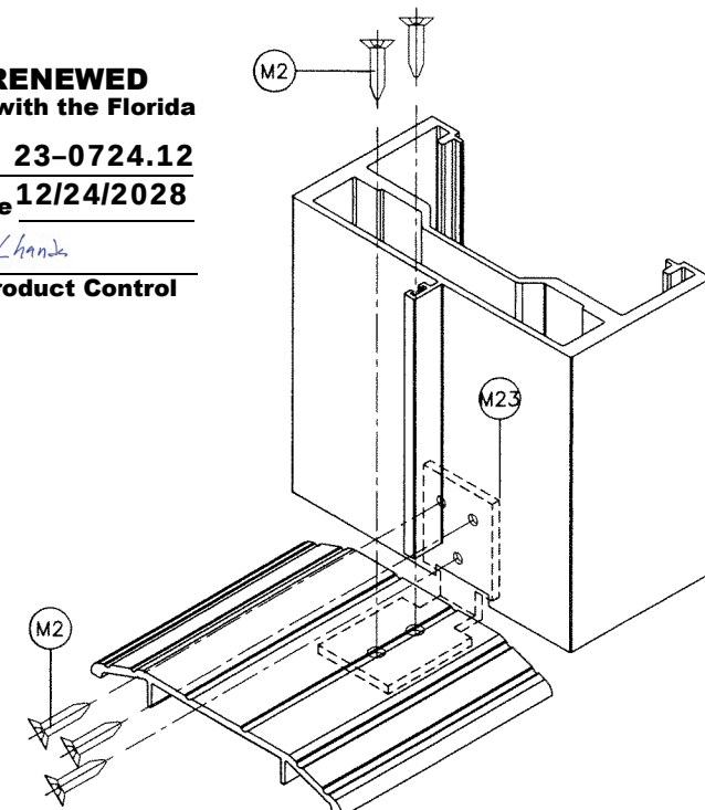
THRESHOLD CORNER
