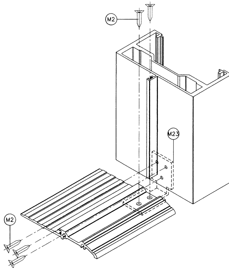
THRESHOLD CORNER
