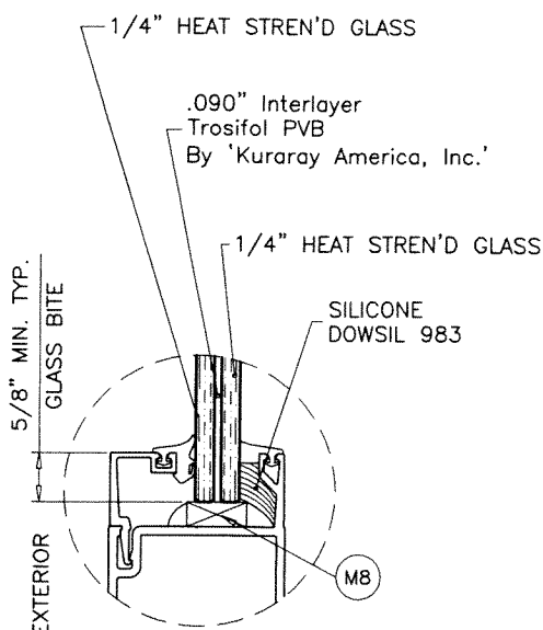
GLASS TYPE 'A.1' 9/16" OVERALL LAM. GLASS
