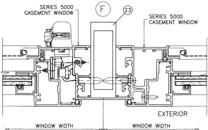
CASEMENT TO CASEMENT MULLION
