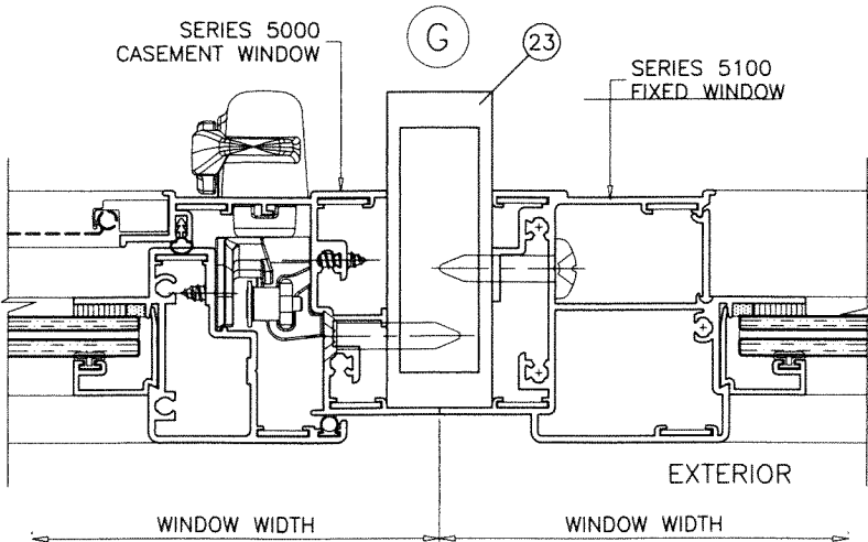
CASEMENT TO FIXED MULLION
