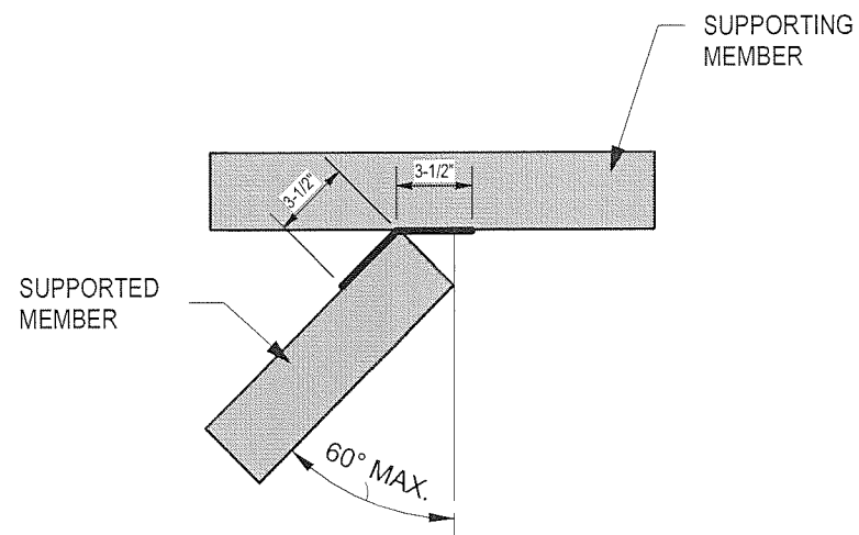
NVSNP3 INSTALLATION
