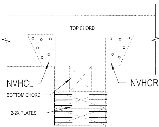
CROSS-SECTION
