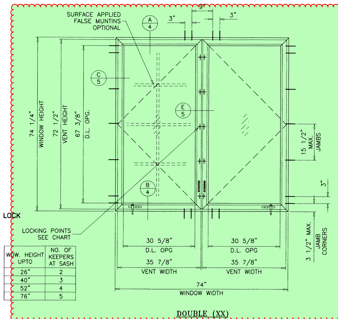
TYPICAL ELEVATIONS
