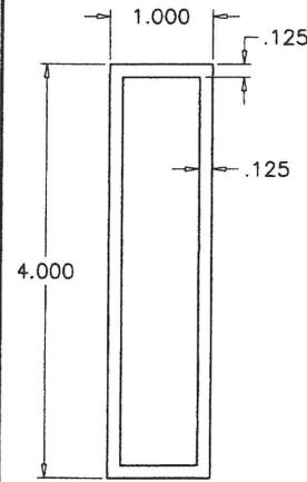
1 X 4 STD. MULLION 6063-T6
