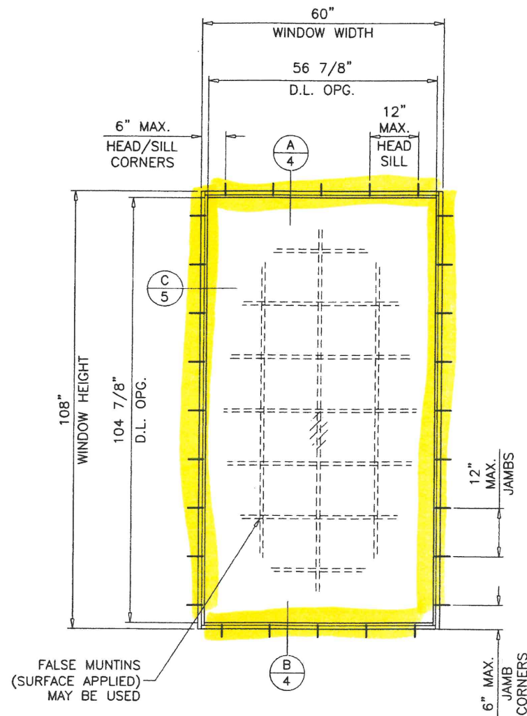
TYPICAL ELEVATION FLANGE FRAMES
