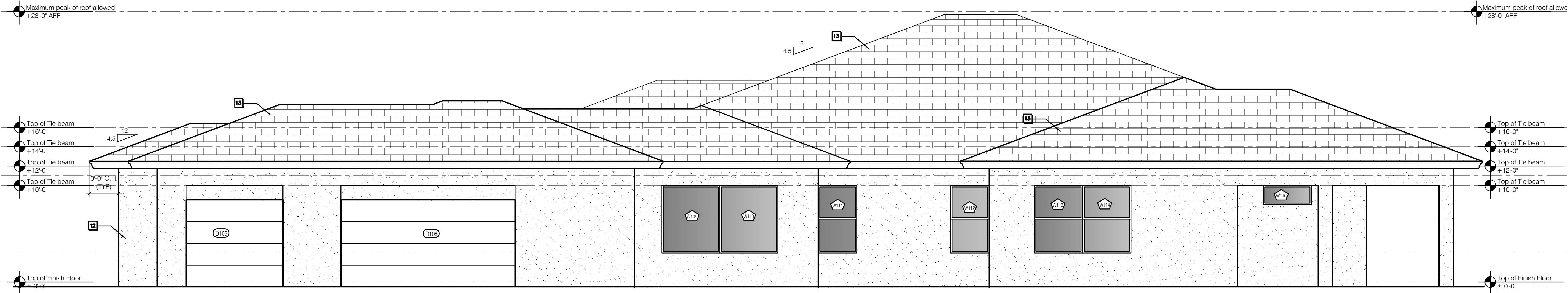
WEST ELEVATION (SIDE) 3/16" SCALE.
