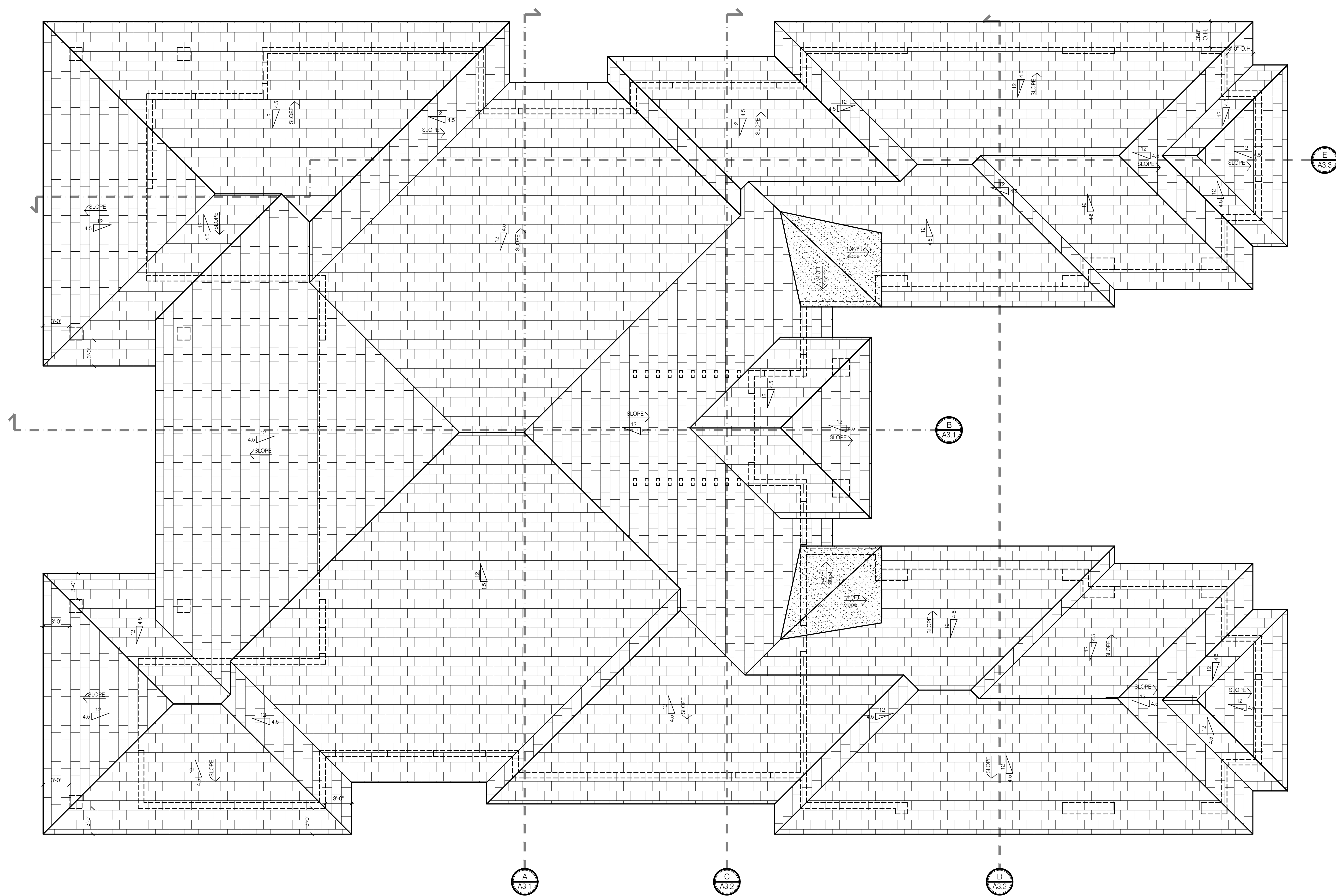
ROOF PLAN 3/16" SCALE.
