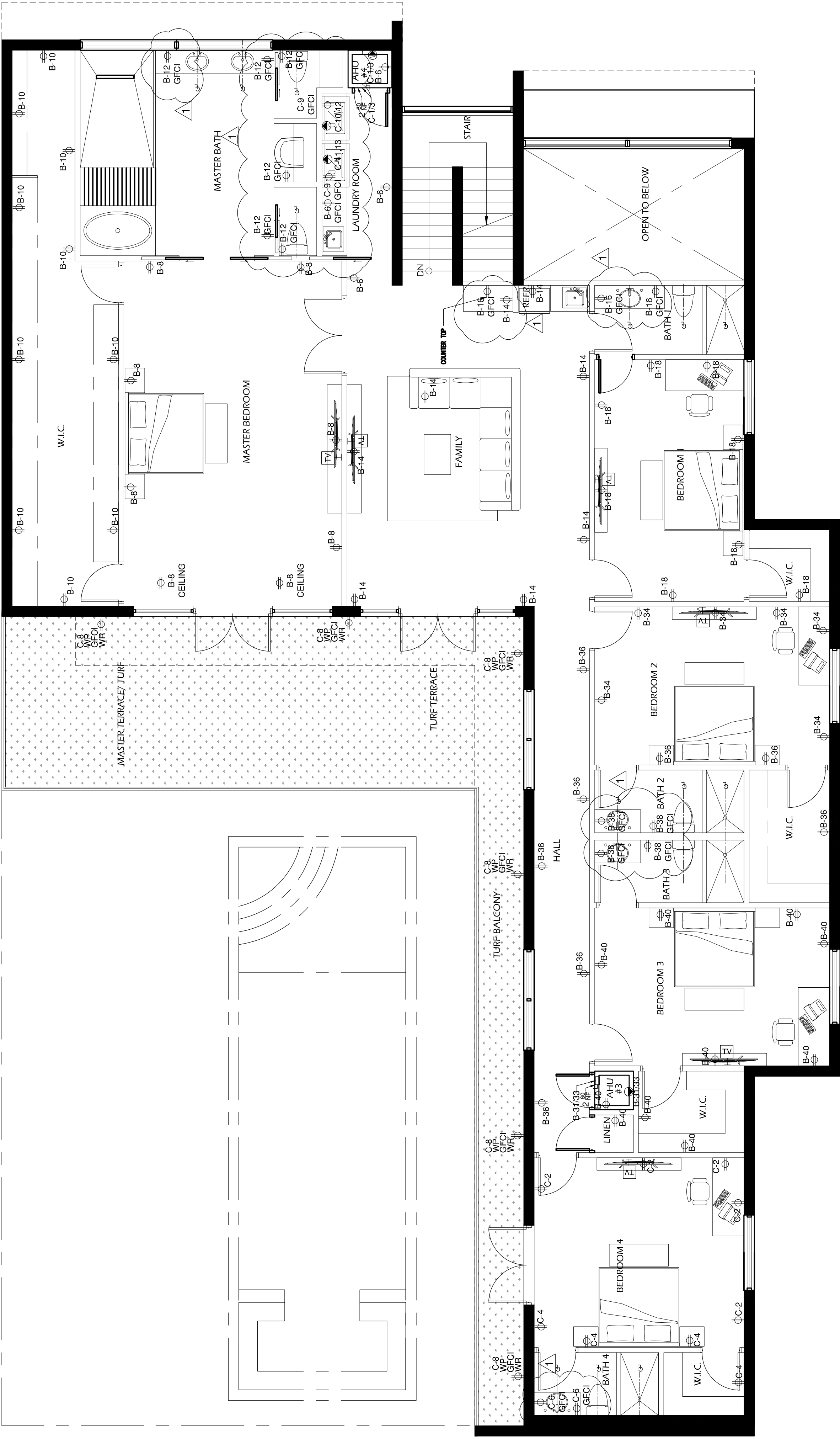
ELECTRICAL SECOND FLOOR PLAN - POWER
