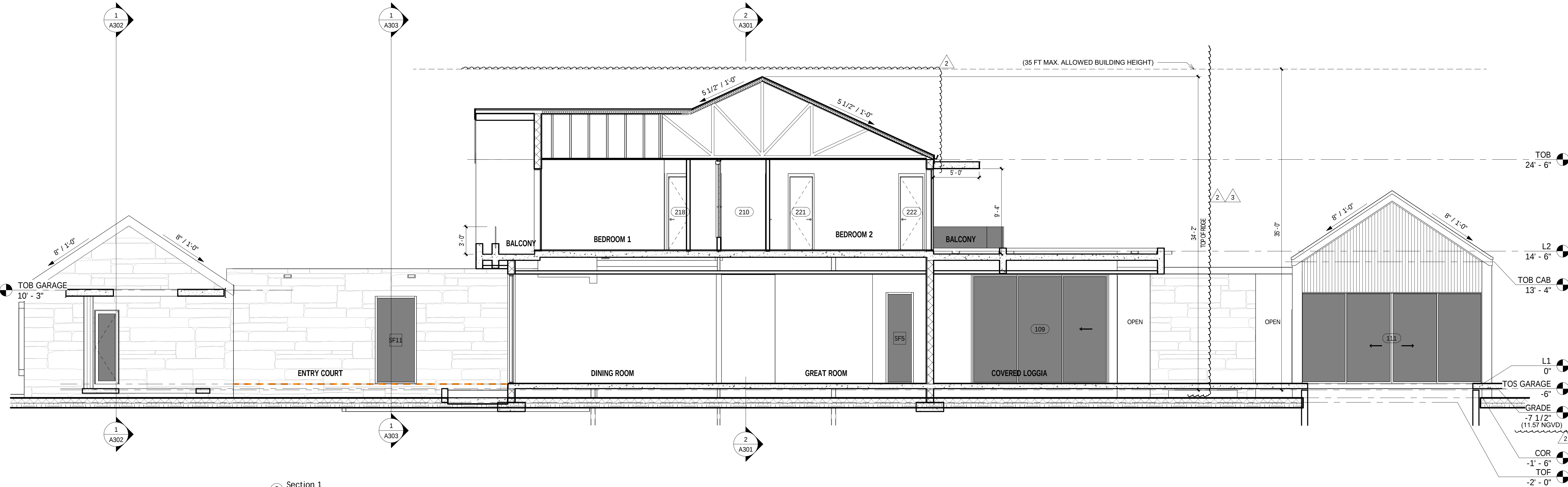
Section 1 3/16" = 1'-0"
