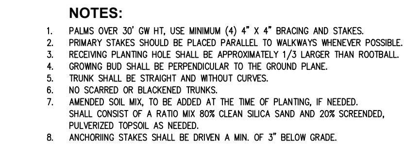
Typical Palm Planting Detail N.T.S.
