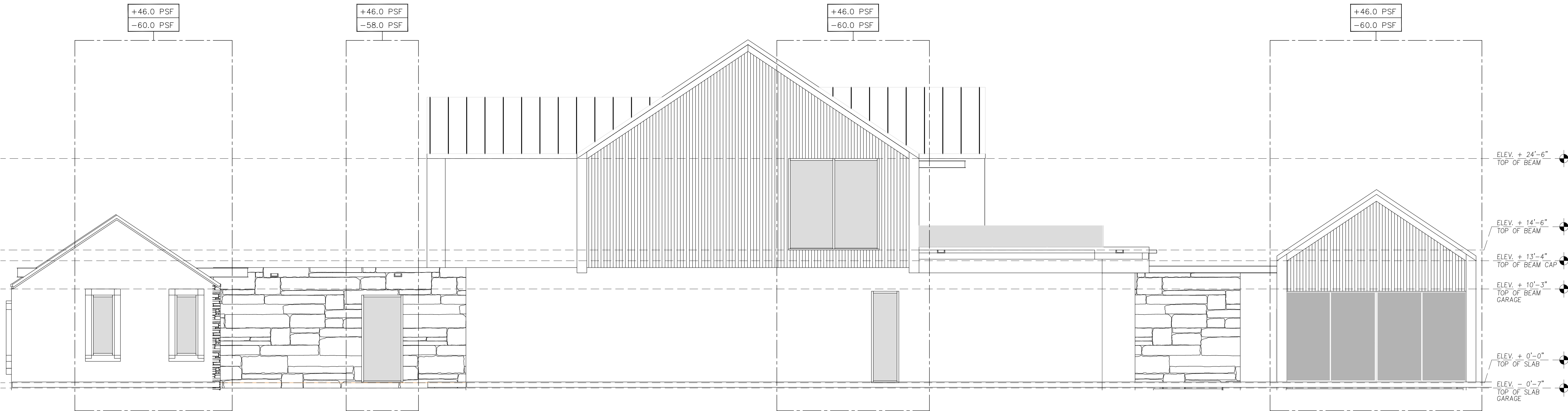
① South Architectural Building Elevation 3/16" = 1'-0"
