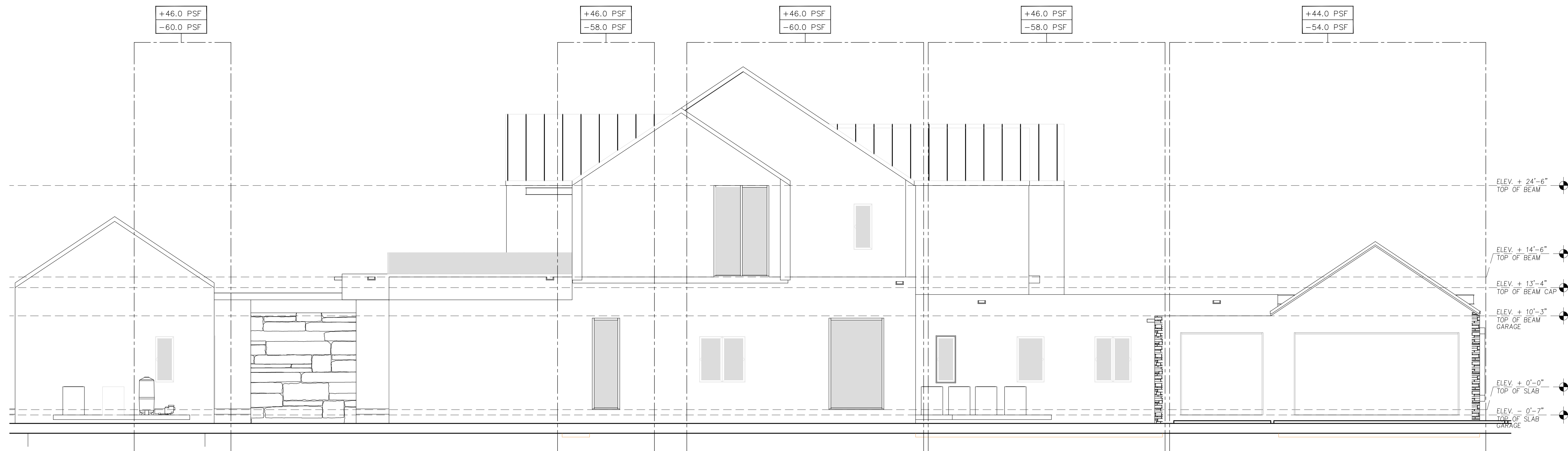
① North Architectural Building Elevation 3/16" = 1'-0"
