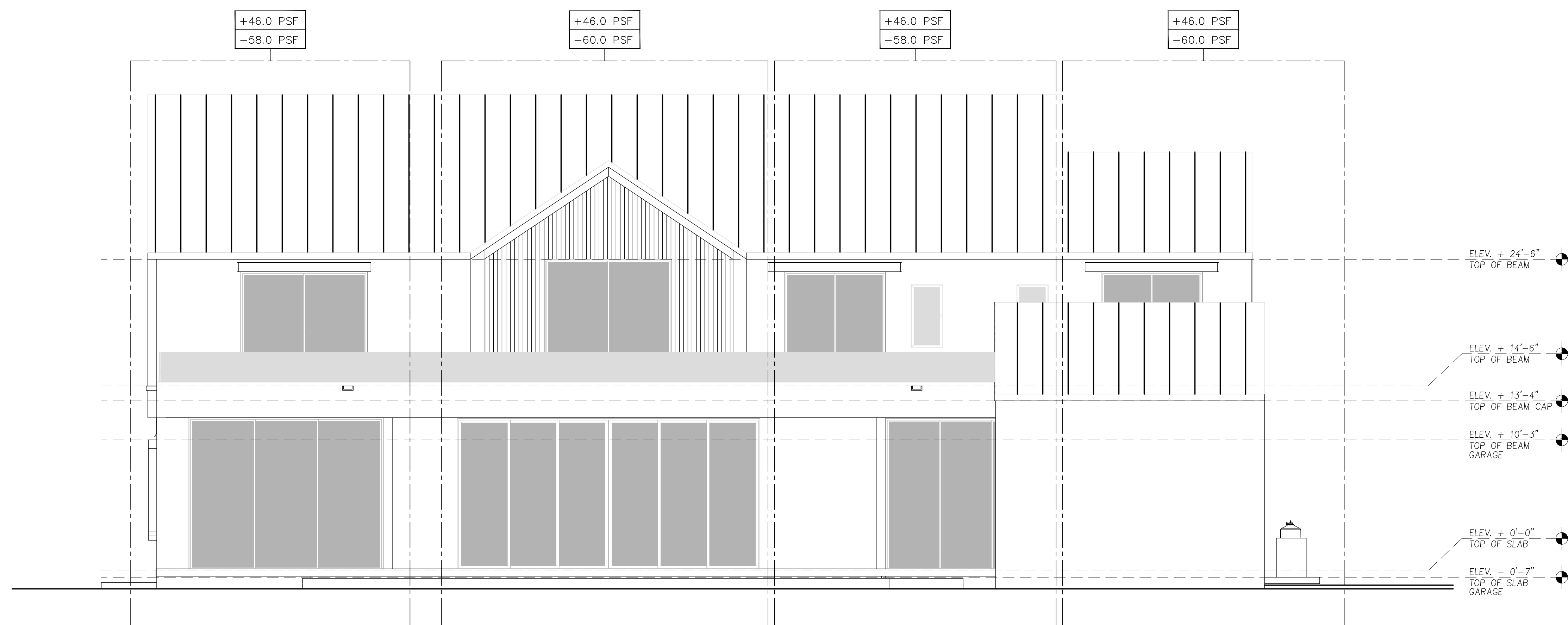
② East Architectural Building Elevation 3/16" = 1'-0"
